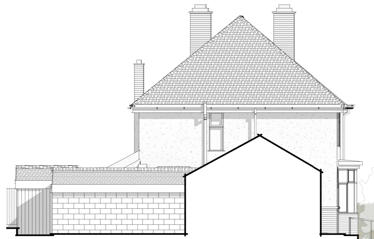
5 | Side Elevation 1 : 100 | A-101
