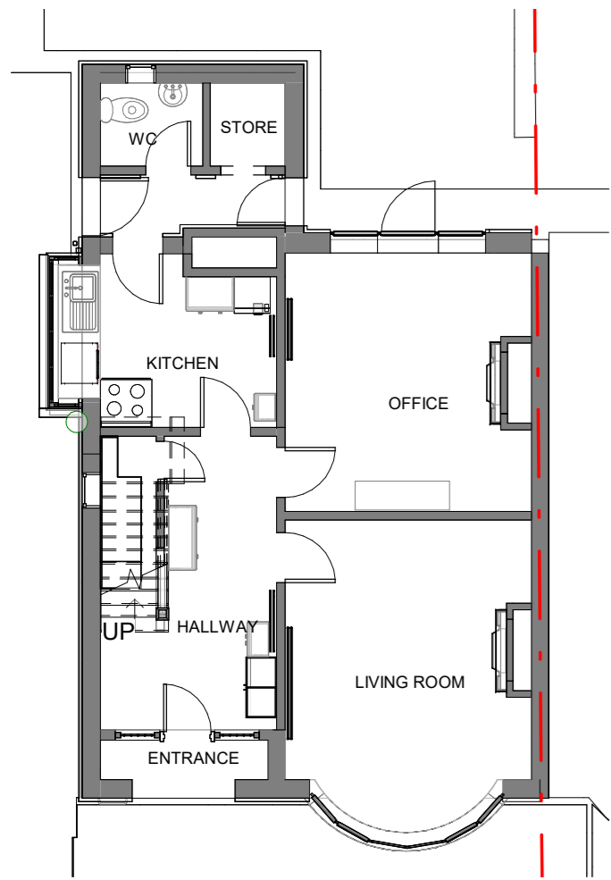
1 | Ground Floor Plan 1 : 100 | A-101
