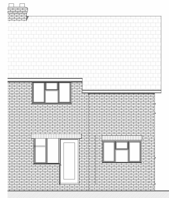
7 West Elevation Original 1 : 100
