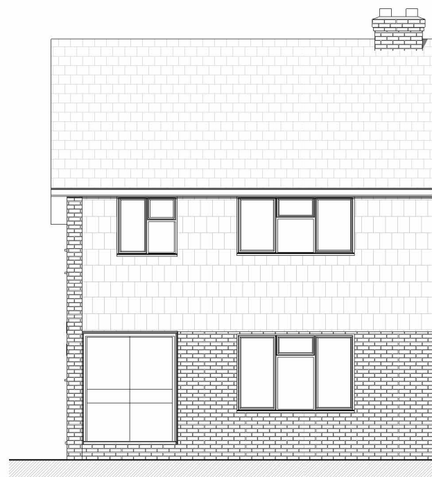
5 East Elevation Original 1 : 100
