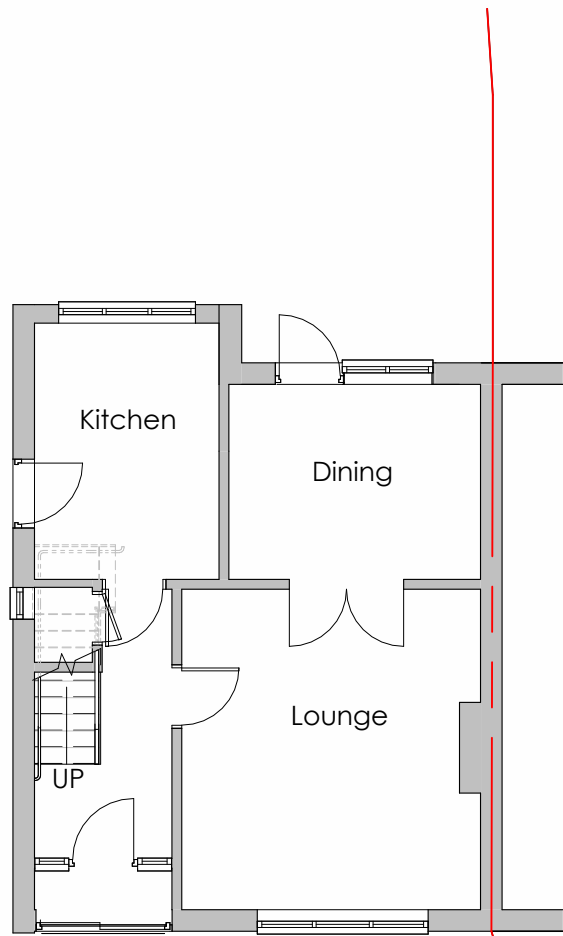
1 Original Ground Floor 1 : 100
