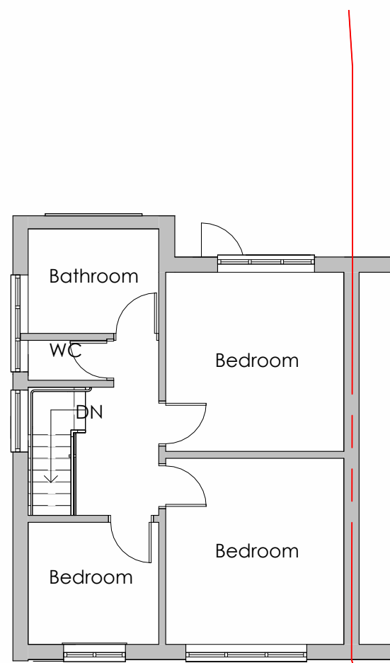
2 Original First Floor Plan 1 : 100
