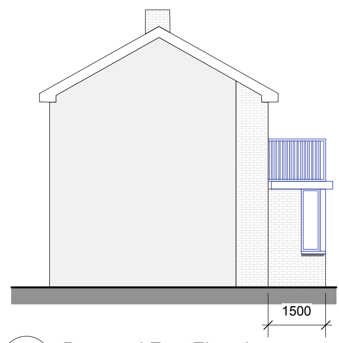
3 Proposed East Elevation 1:100 @ A3
