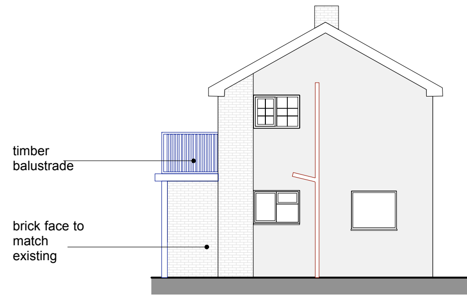
4 Proposed West Elevation 1:100 @ A3
