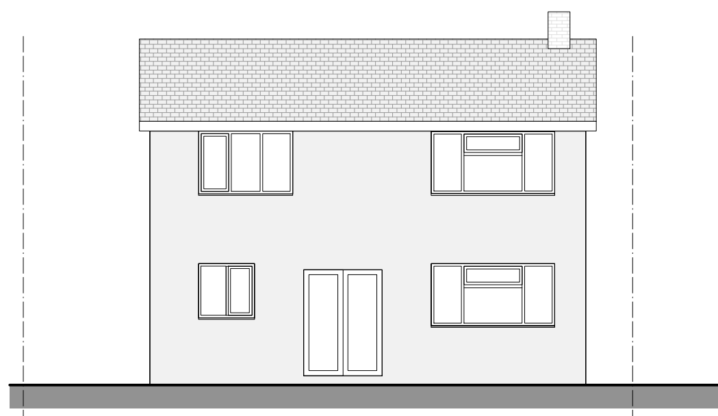
2 Proposed South Elevation 1:100 @ A3
