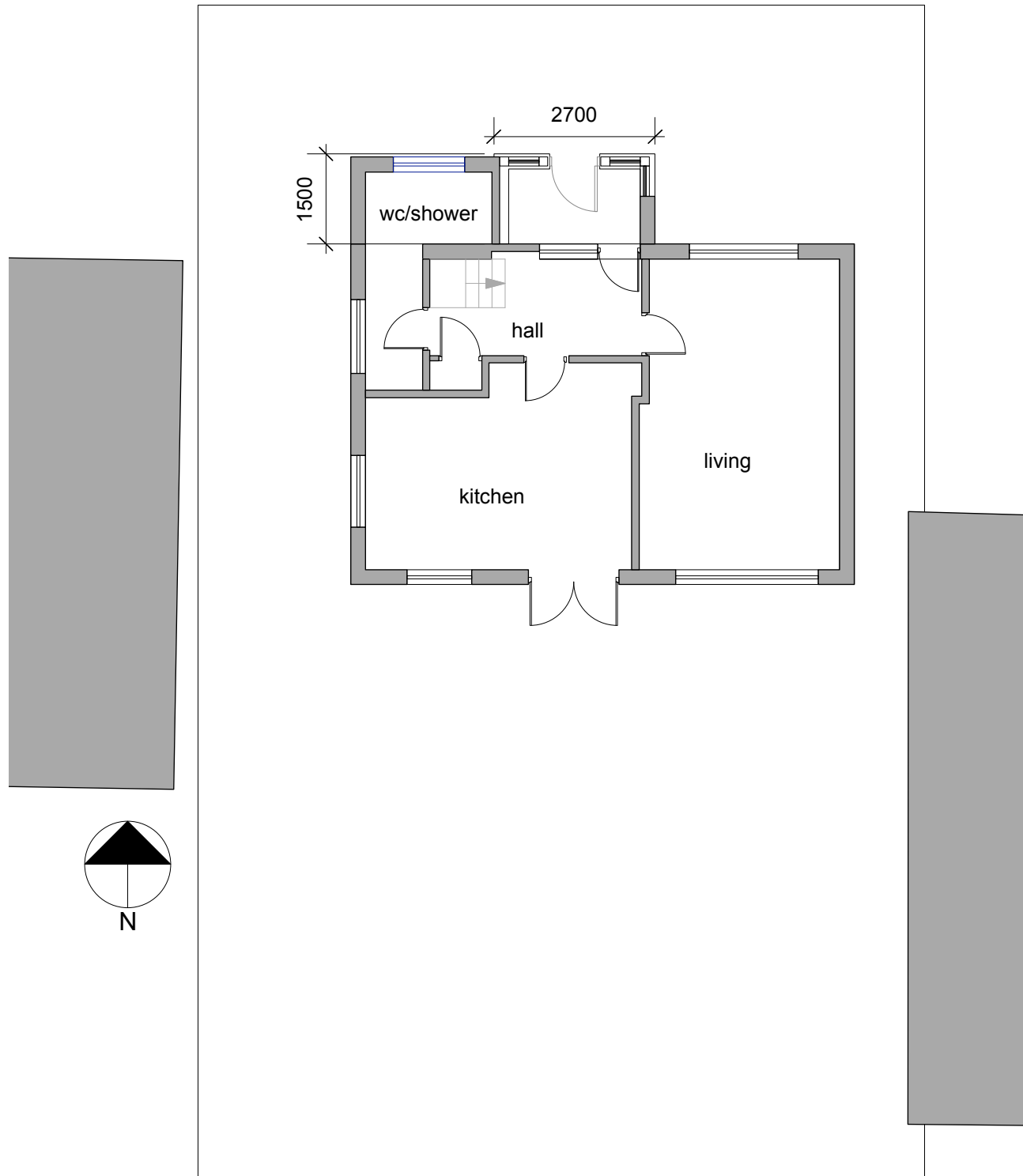
1 Proposed Ground floor 1:100 @ A3
