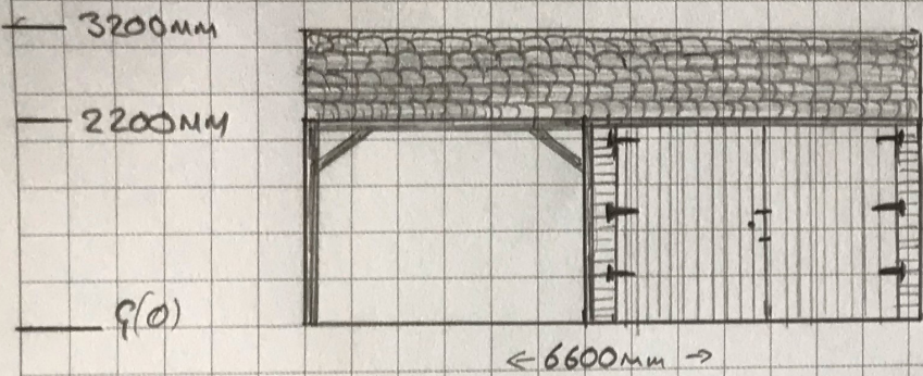
FRONT ELEVATION (FACING NORTH)
