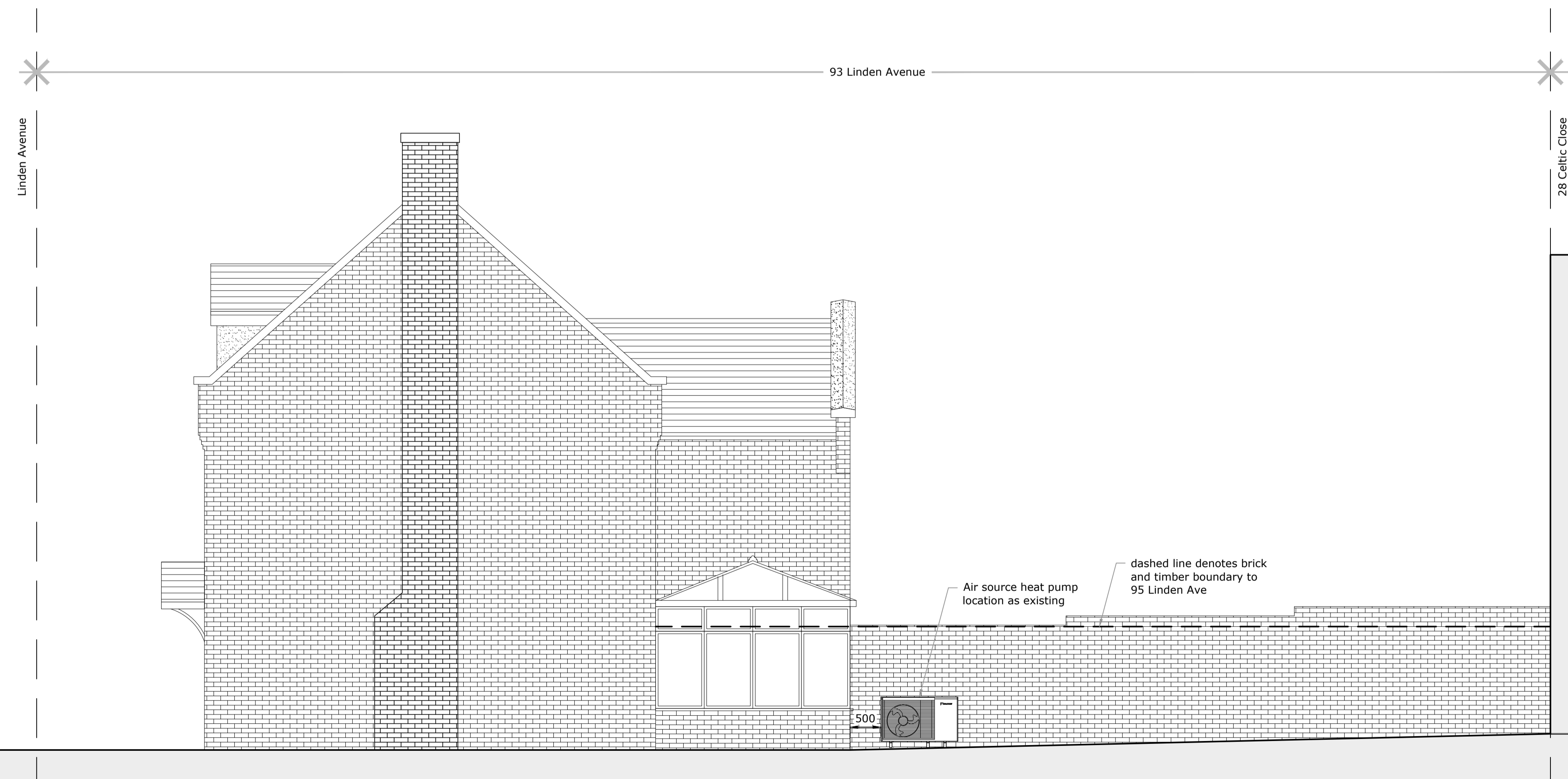
side elevation (north west facing) as existing 1:50
