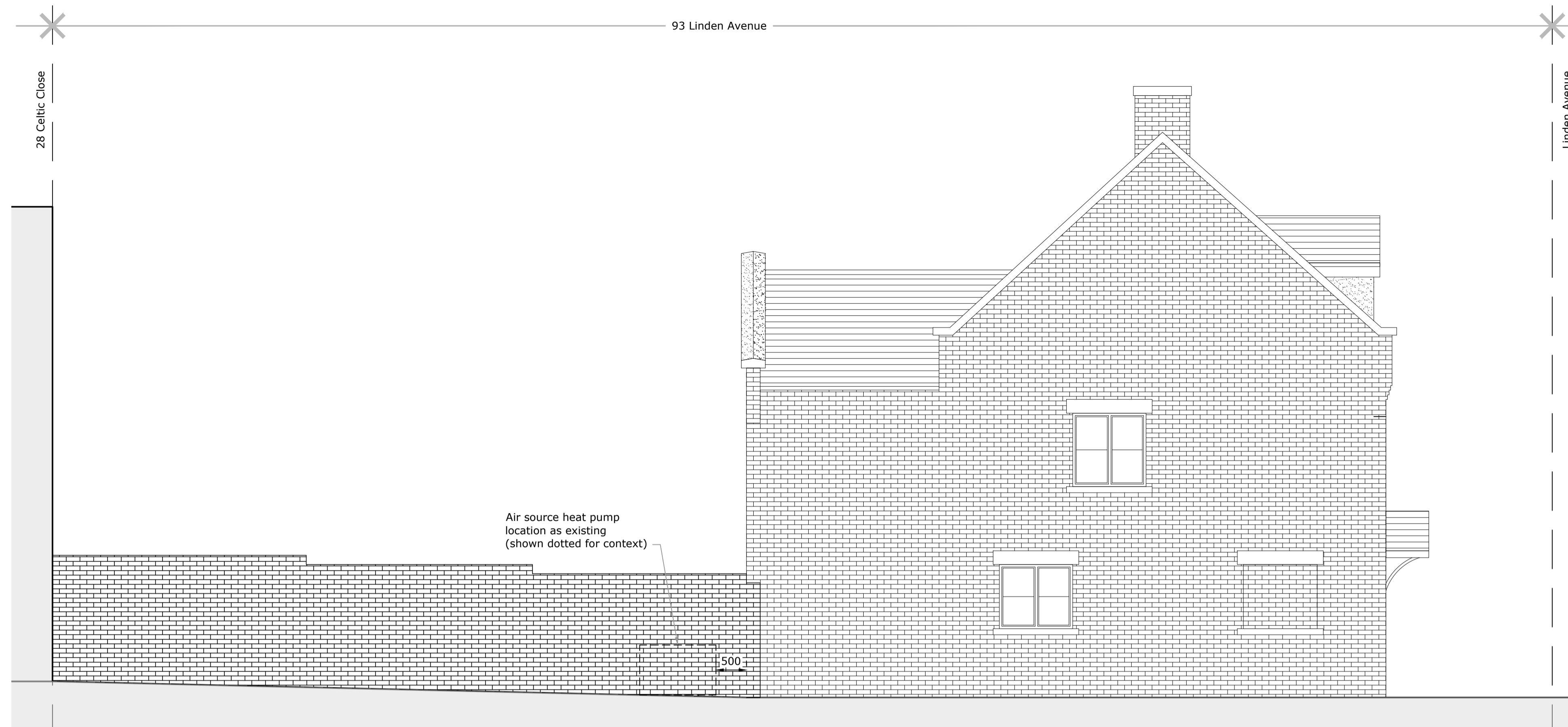
side elevation (south east facing) as existing 1:50
