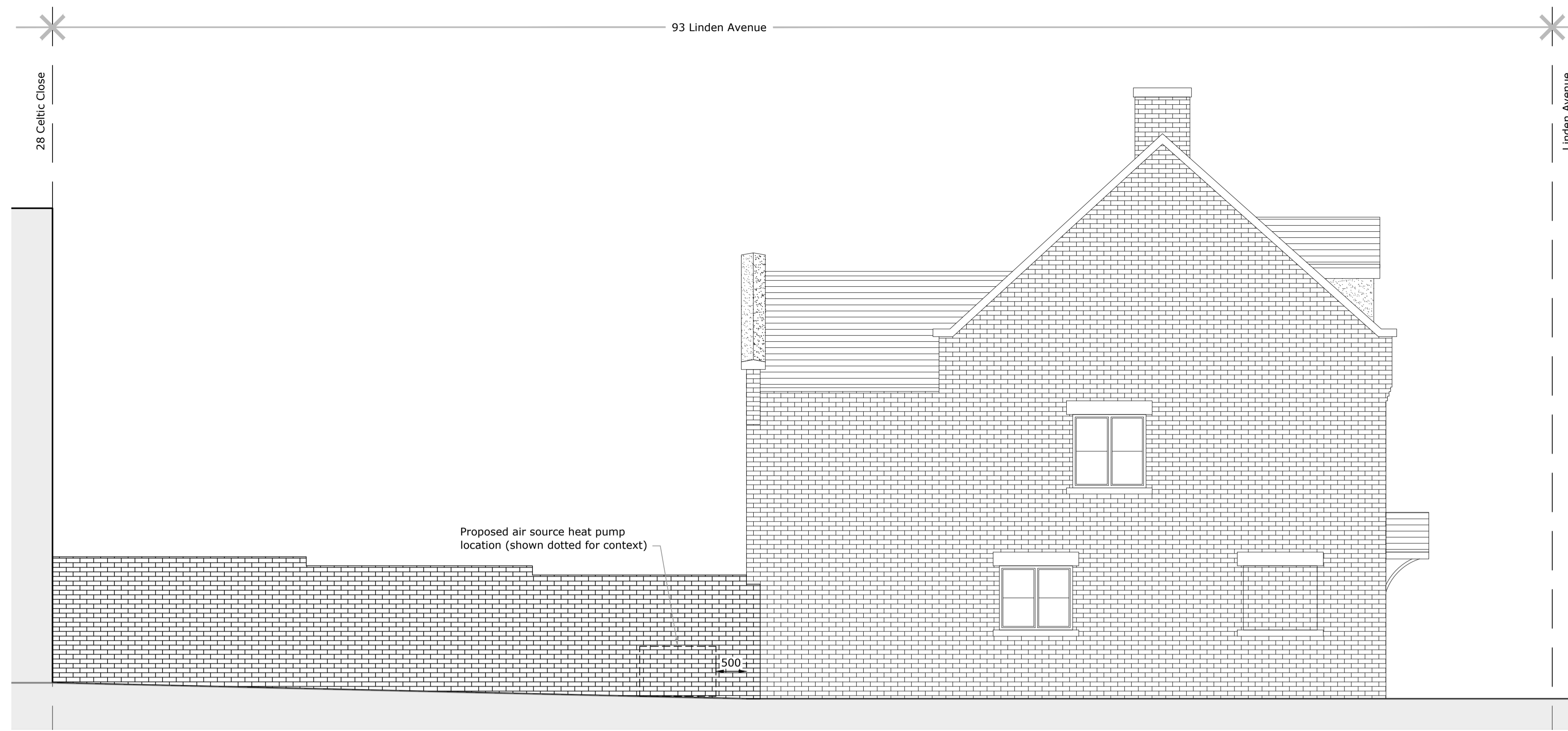
side elevation (south east facing) as proposed 1:50
