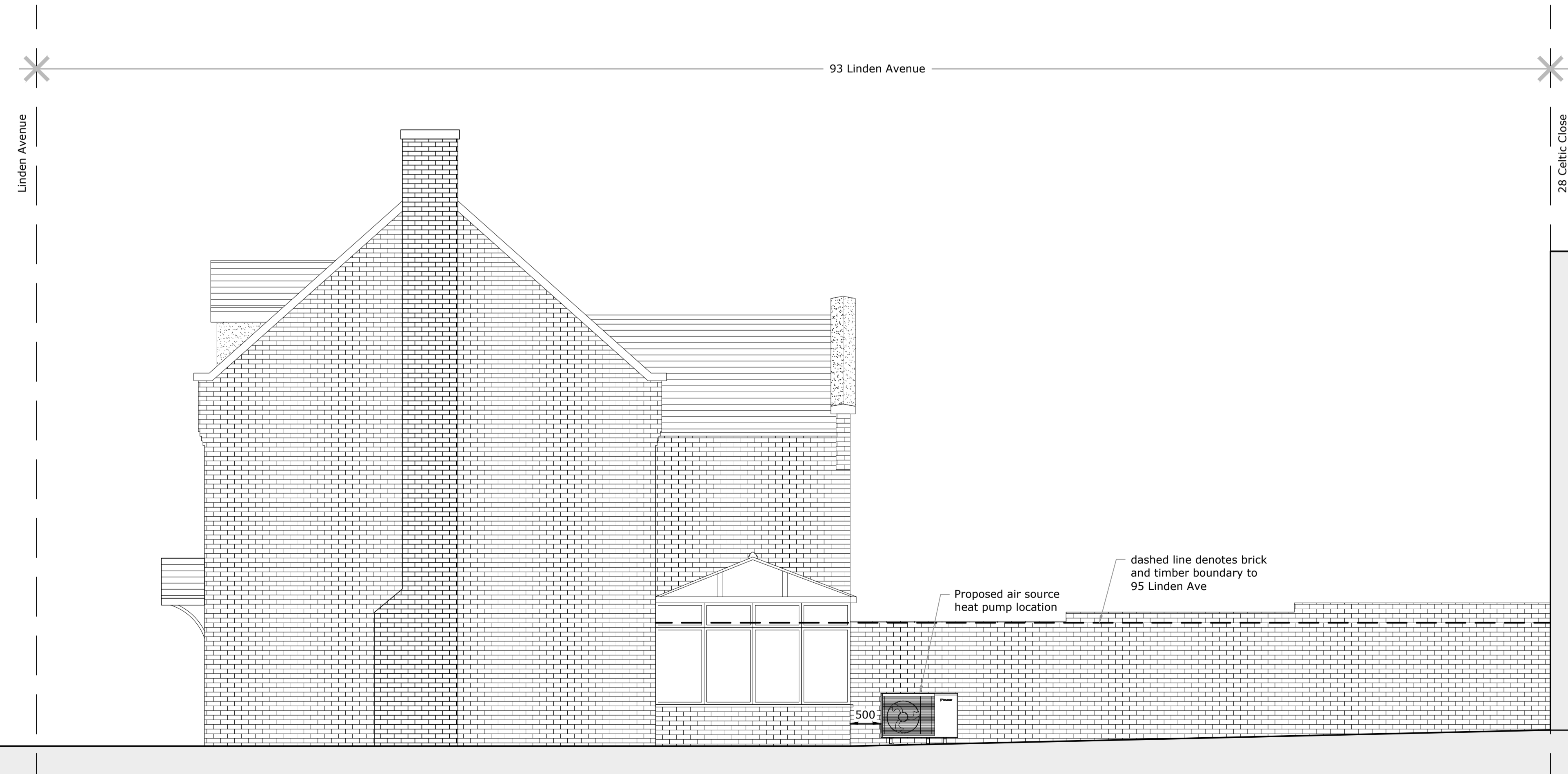
side elevation (north west facing) as proposed 1:50
