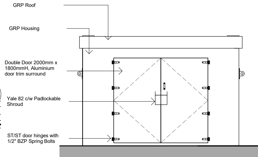
A Substation, front elevation, as proposed 1 : 50
