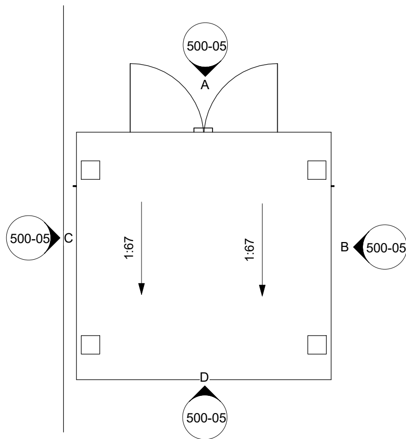
HV substation, roof plan, as proposed 1 : 50
