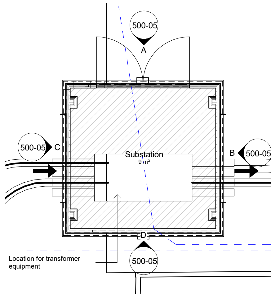
HV substation, as proposed 1 : 50
