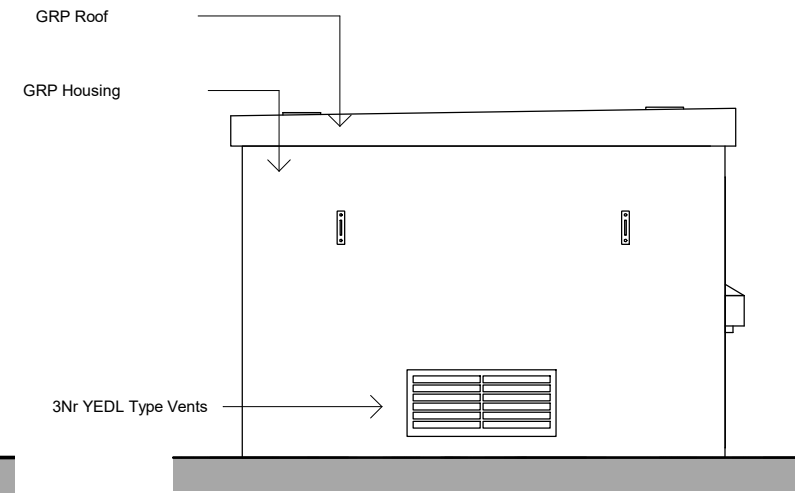
B Substation, East elevation, as proposed 1 : 50
