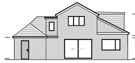
PROPOSED REAR ELEVATION EAST FACING
