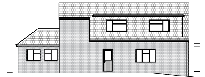
EXISTING SIDE ELEVATION NORTH FACING
