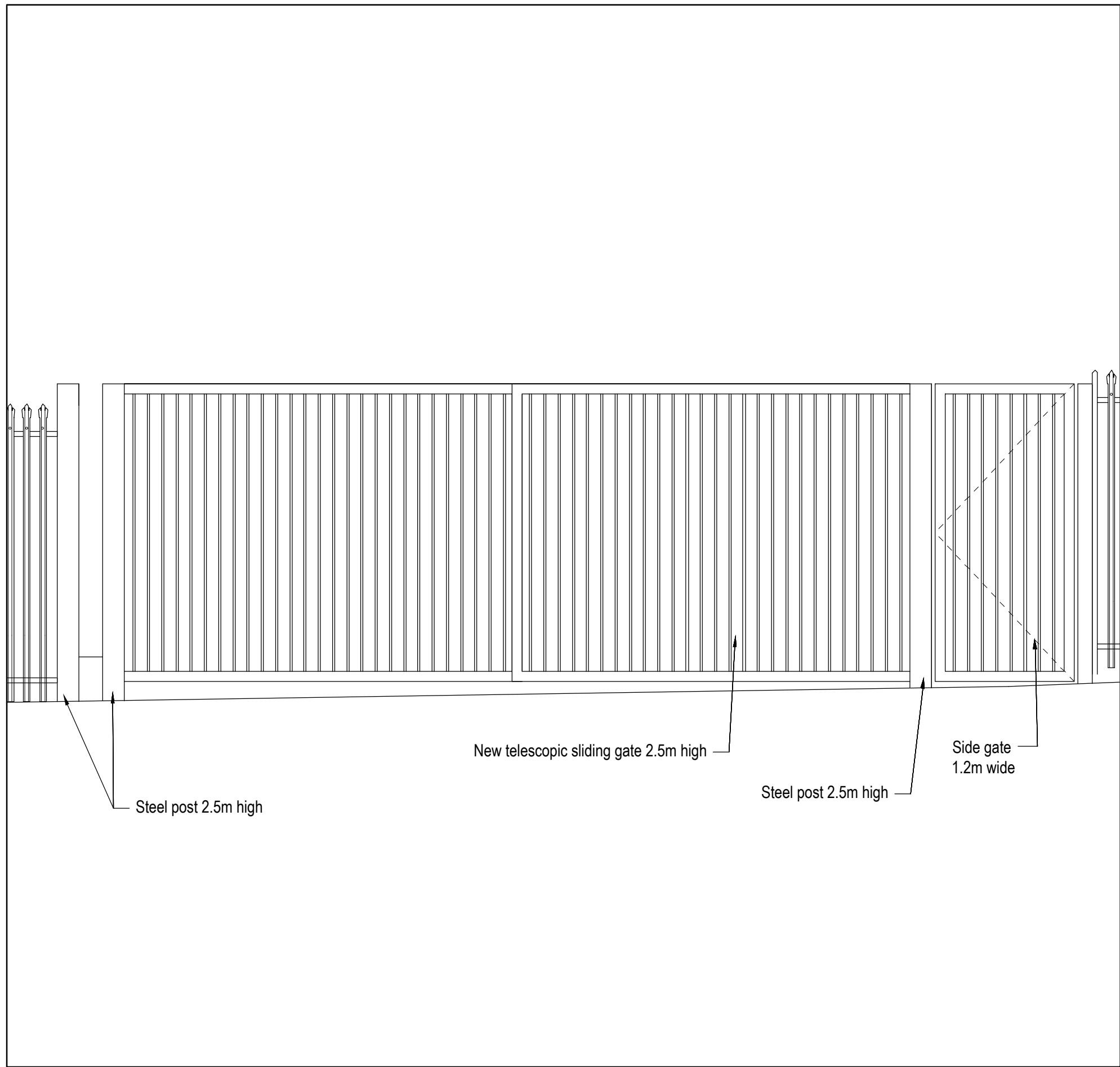
GATE ELEVATION SCALE 1:35
