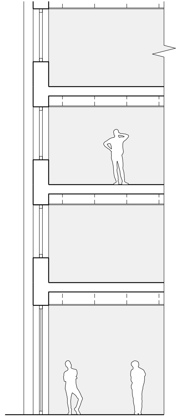
01 DRG Proposed Section 1:75@A3
