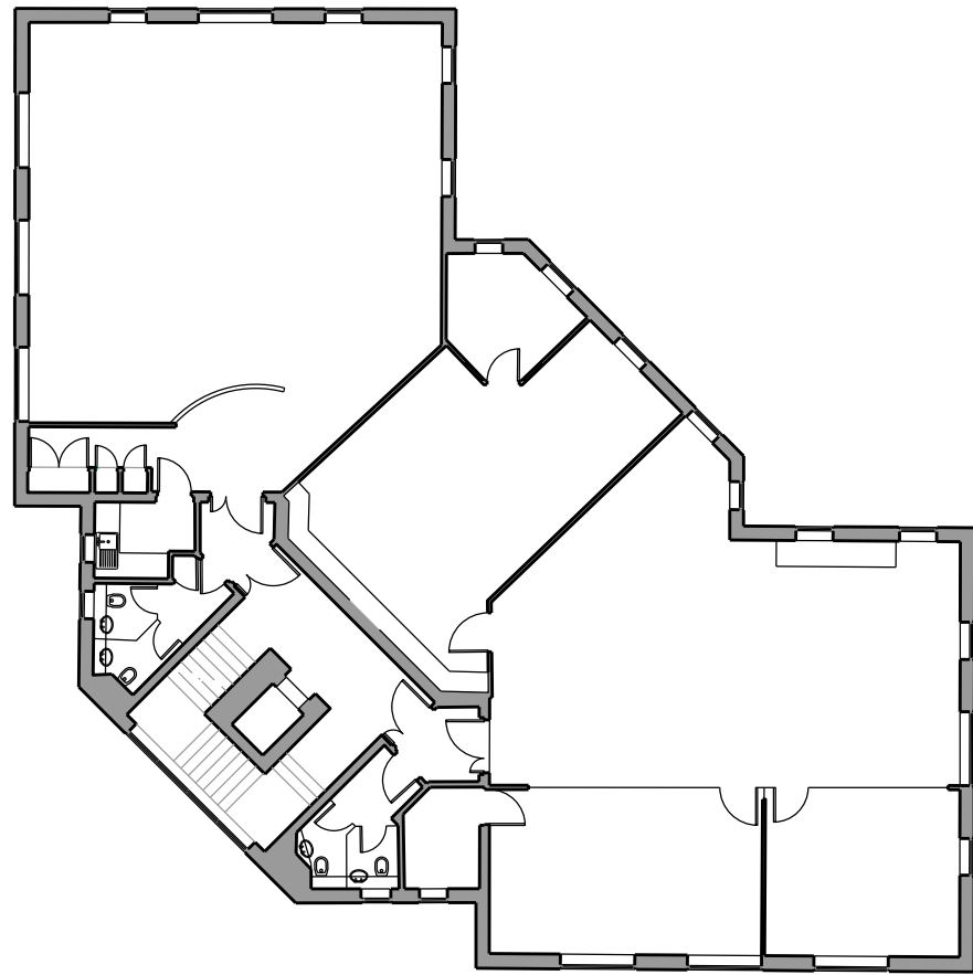
First Floor Plan 1:200@A3
