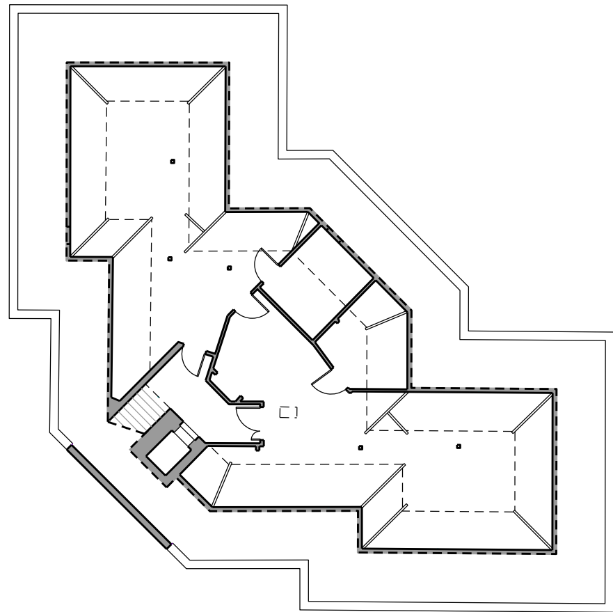
Third Floor Plan 1:200@A3
