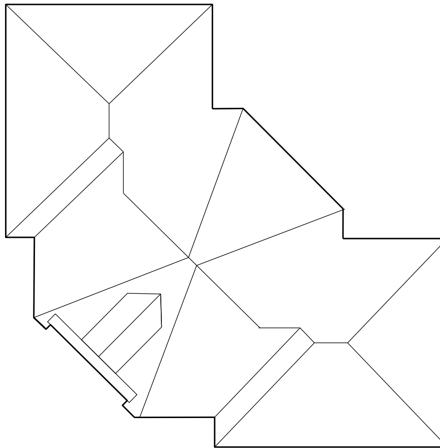
Roof Plan 1:200@A3
