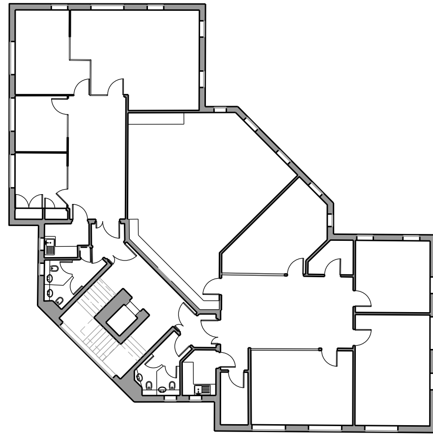
Second Floor Plan 1:200@A3
