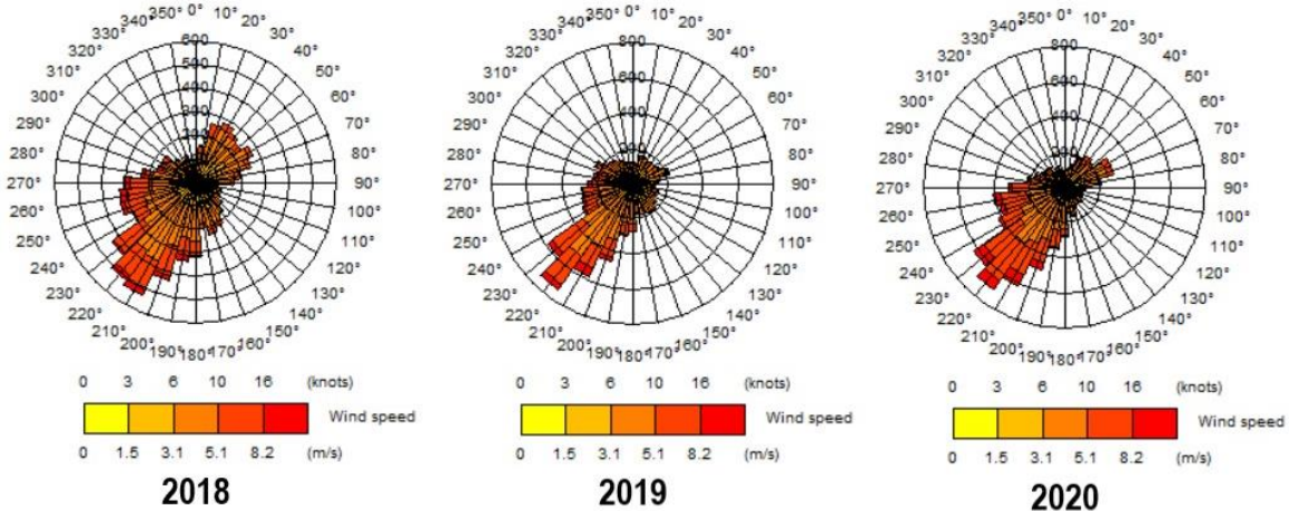
Figure 3.3: Windrose for Kenley Airfield Meteorological Station 2018-2020
