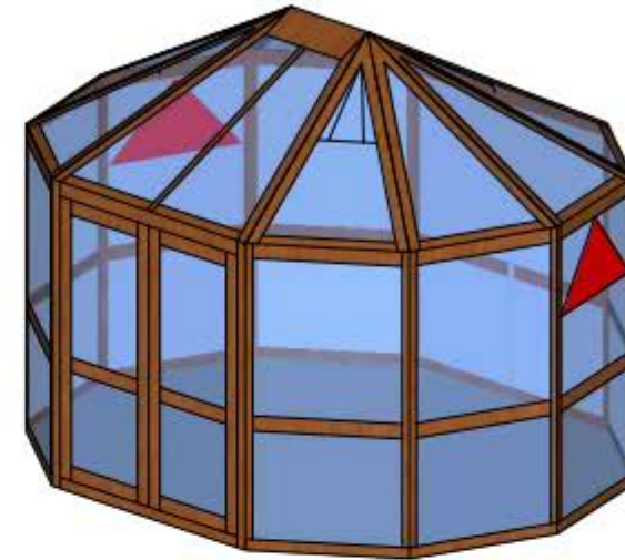
ISOMETRIC VIEW
