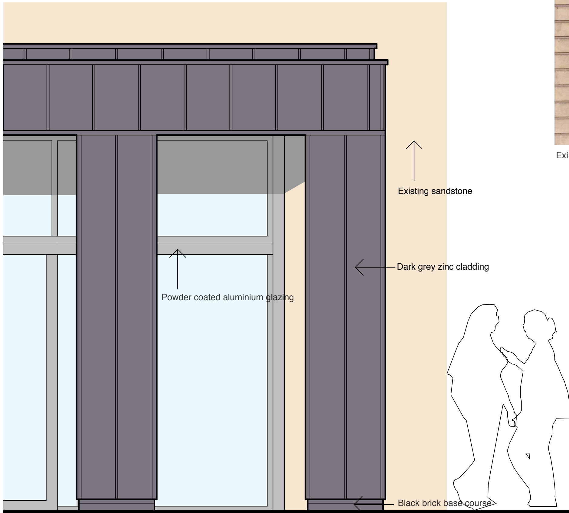
Canopy cladding detail 1:20
