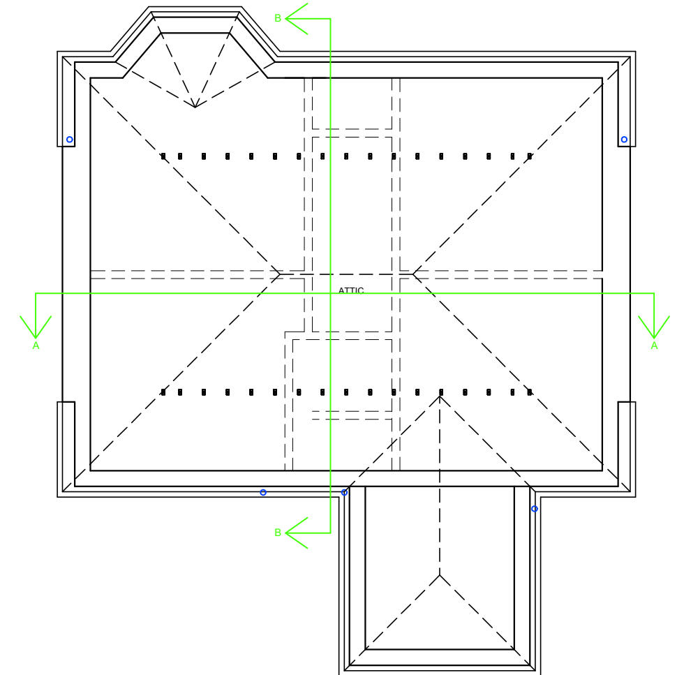
EXISTING ATTIC FLOOR PLAN
