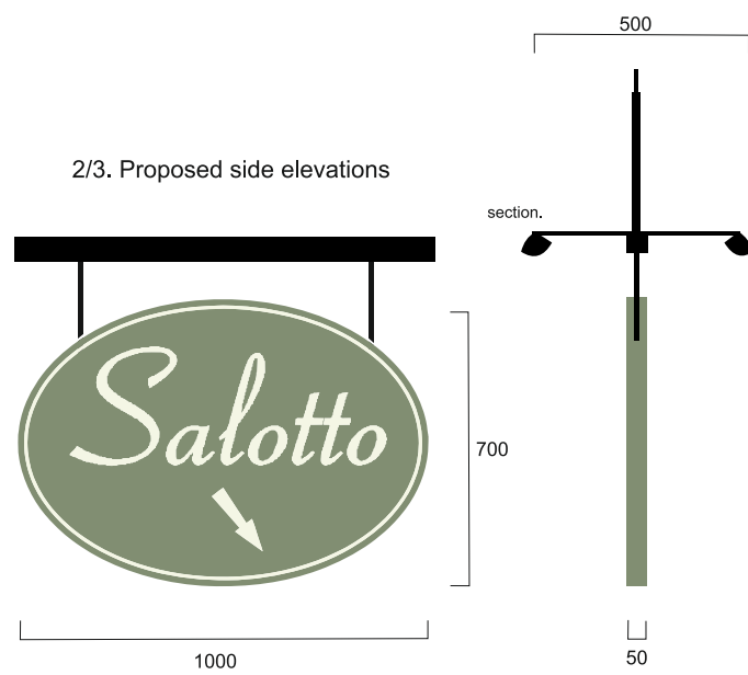
2/3. Proposed side elevations 1:20 @ A3
