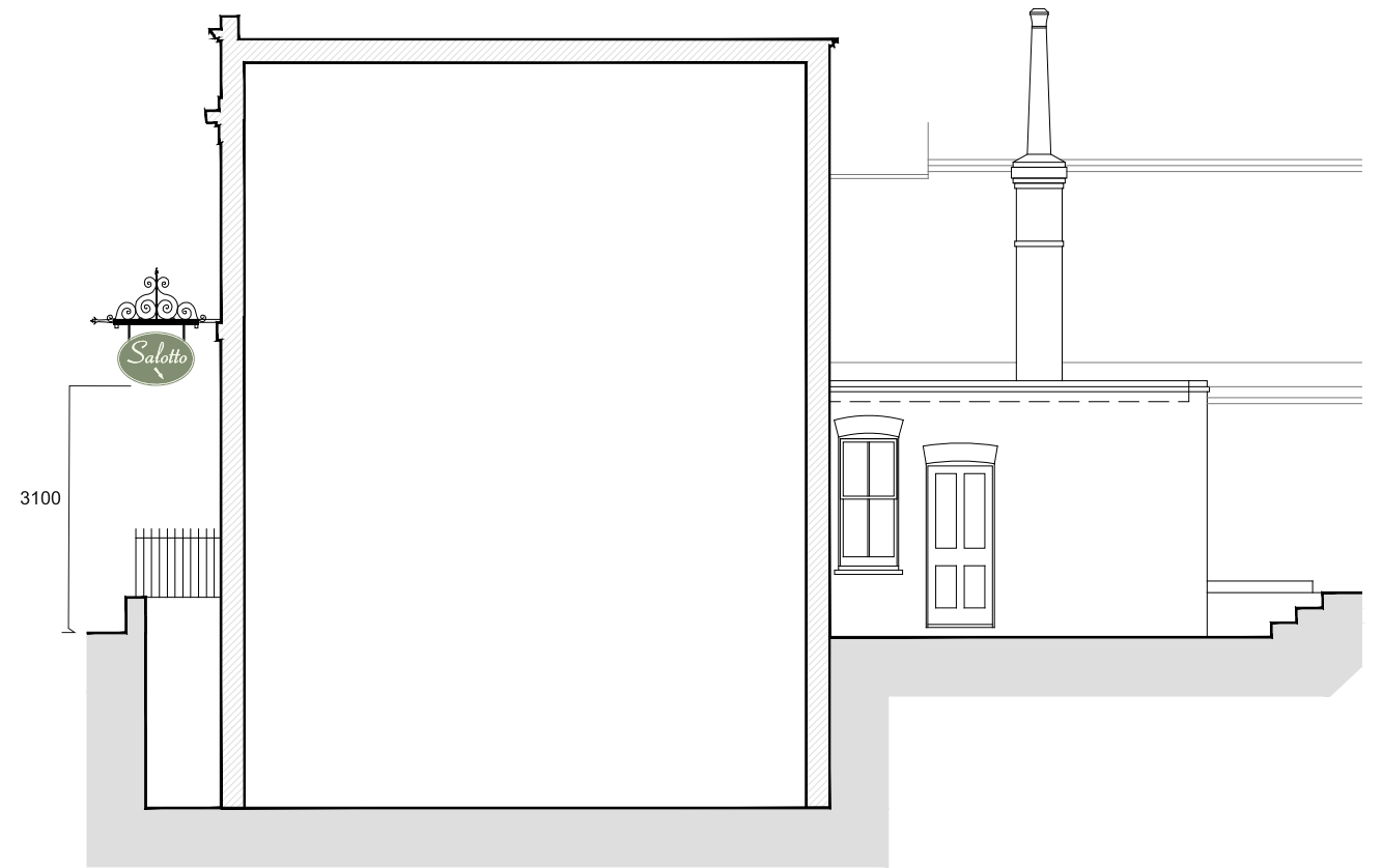
3. Proposed side elevation 1:100 @ A3
