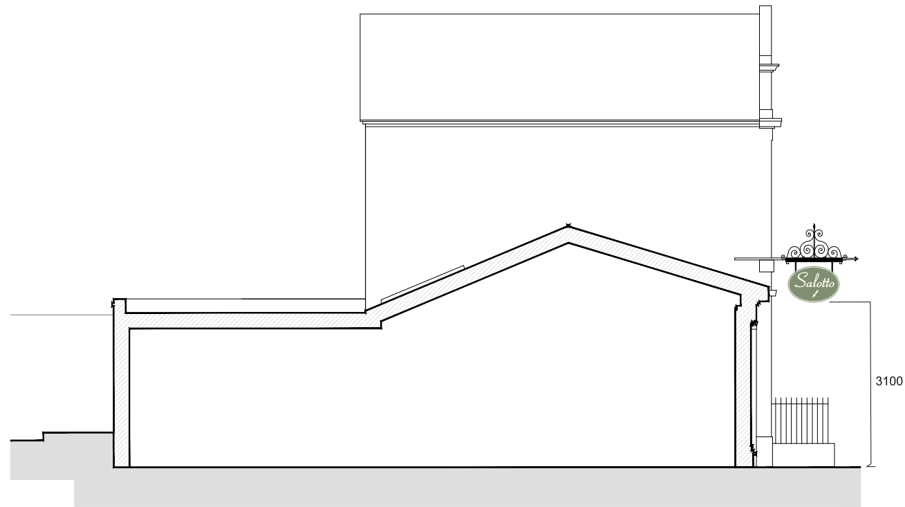
2. Proposed side elevation 1:100 @ A3
