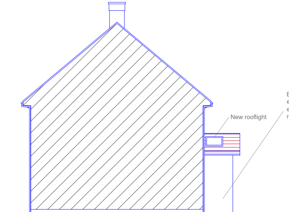
SIDE ELEVATION (WEST): AS PROPOSED
