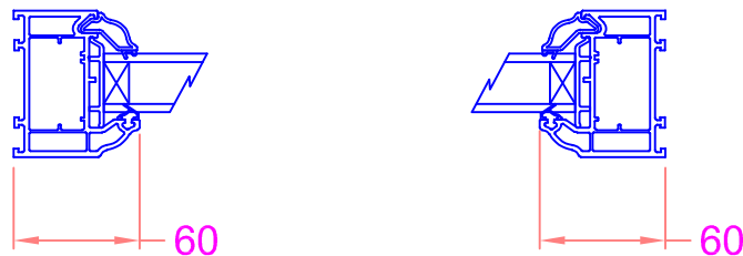
Section V-V Scale 1:4
