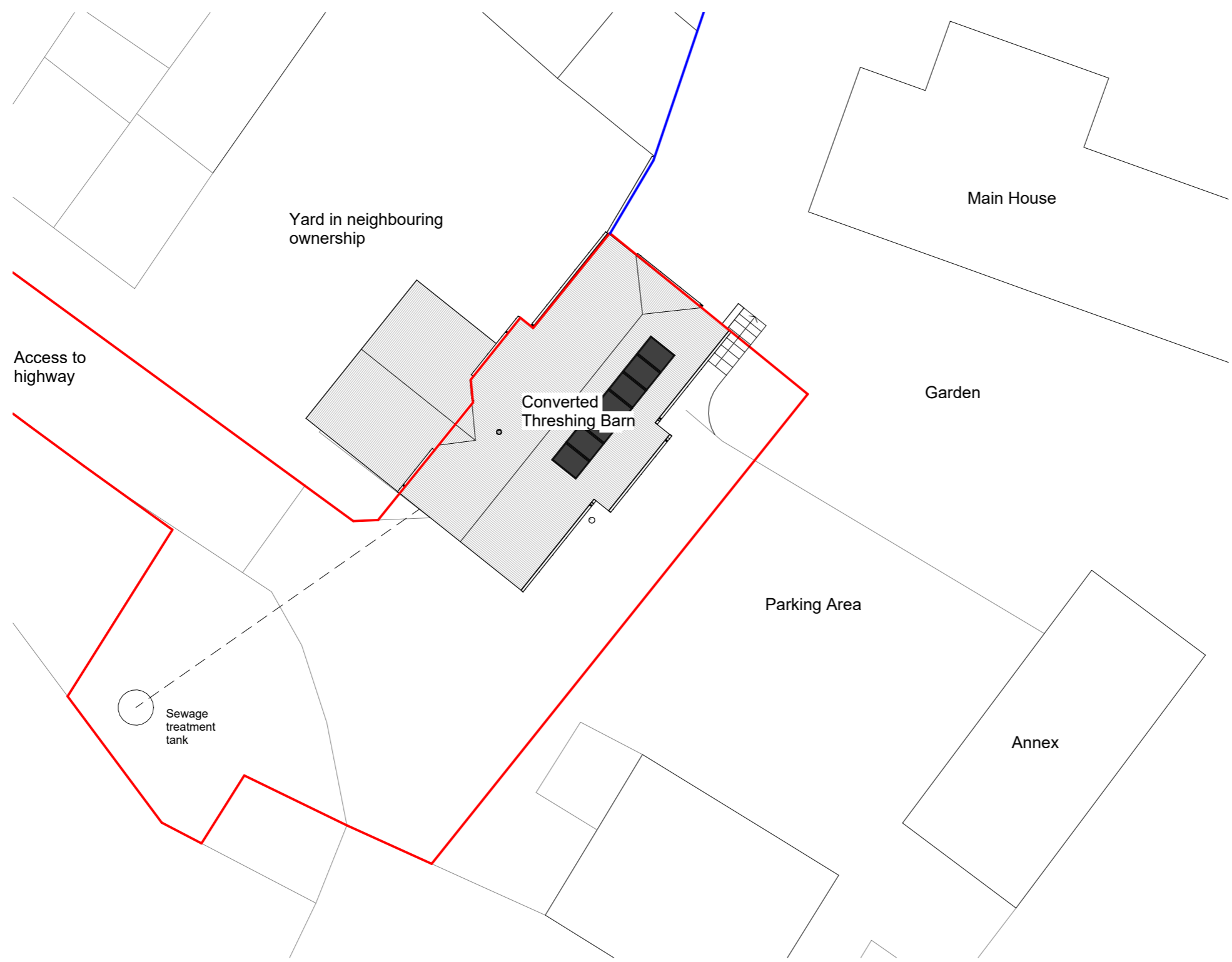
1 Proposed Block Plan 1 : 200
