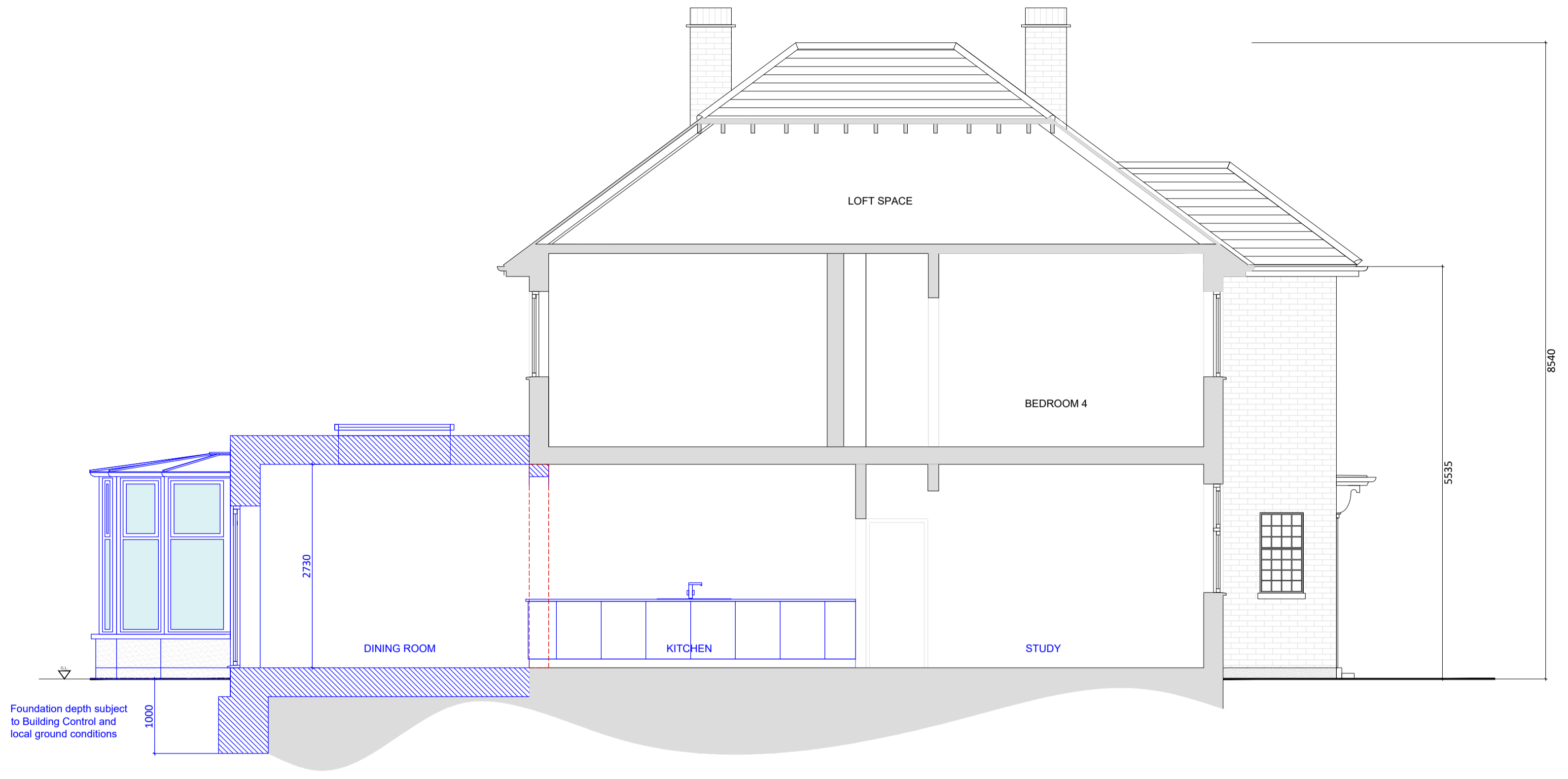
PROPOSED SECTION A-A SCALE: 1:50
