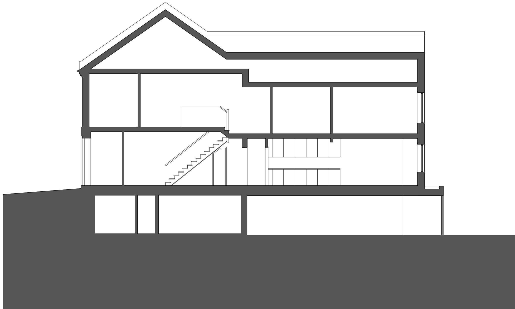
01 Proposed Section CC Scale: 1:100
