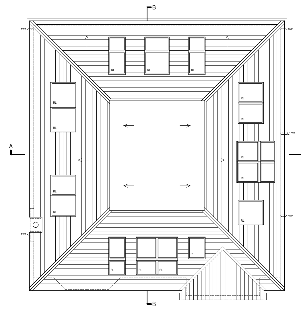
Roof Plan as Proposed
