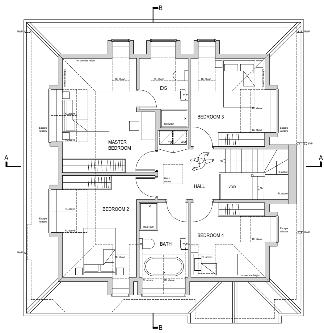
Upper Floor Plan as Proposed
