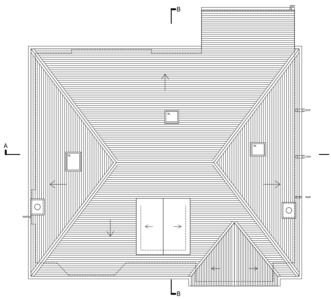
Roof Plan as Existing
