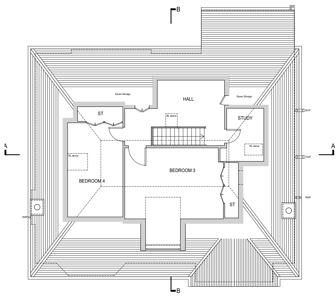
Upper Floor Plan as Existing
