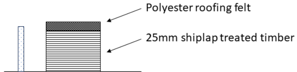
East 1:100
