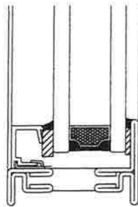
INTERNALLY GLAZED
