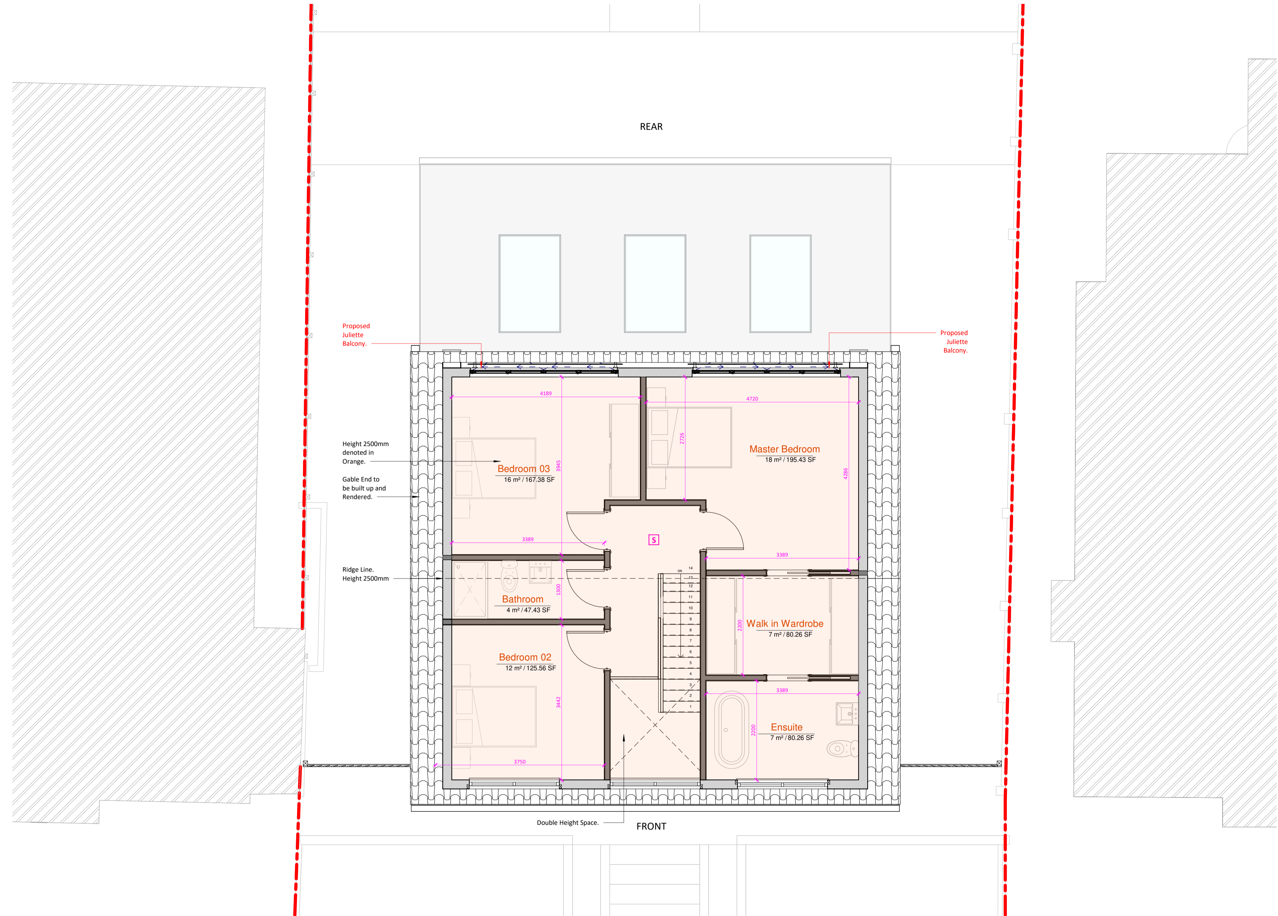
1 Proposed Loft Plan 1 : 50
