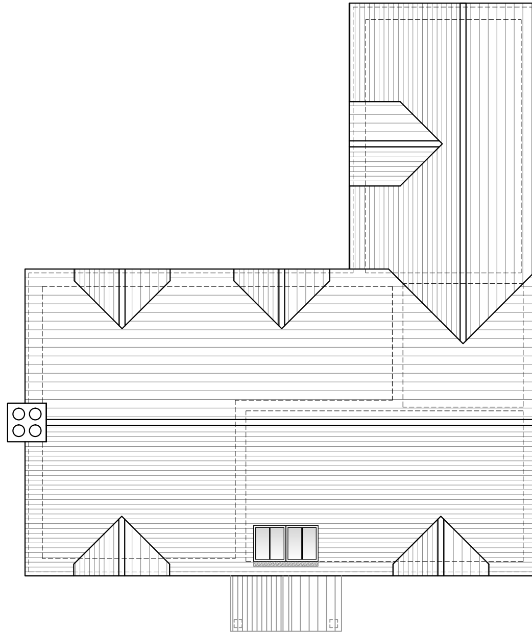
ROOF PLAN
