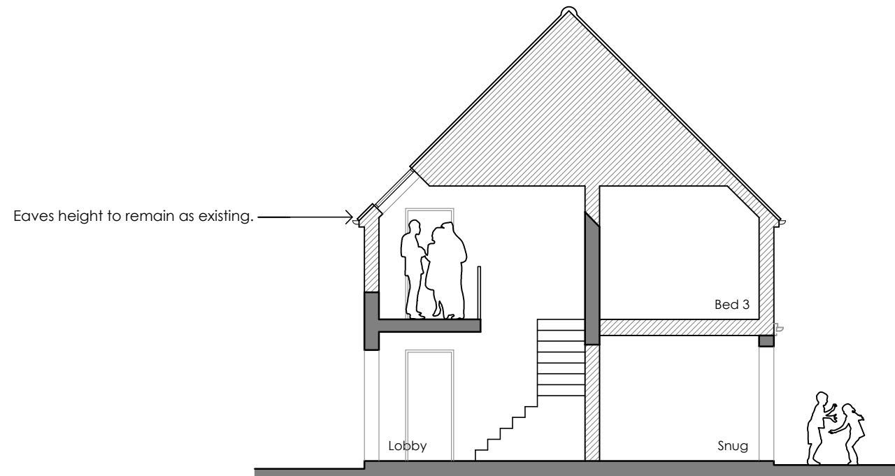
TYPICAL SECTION
