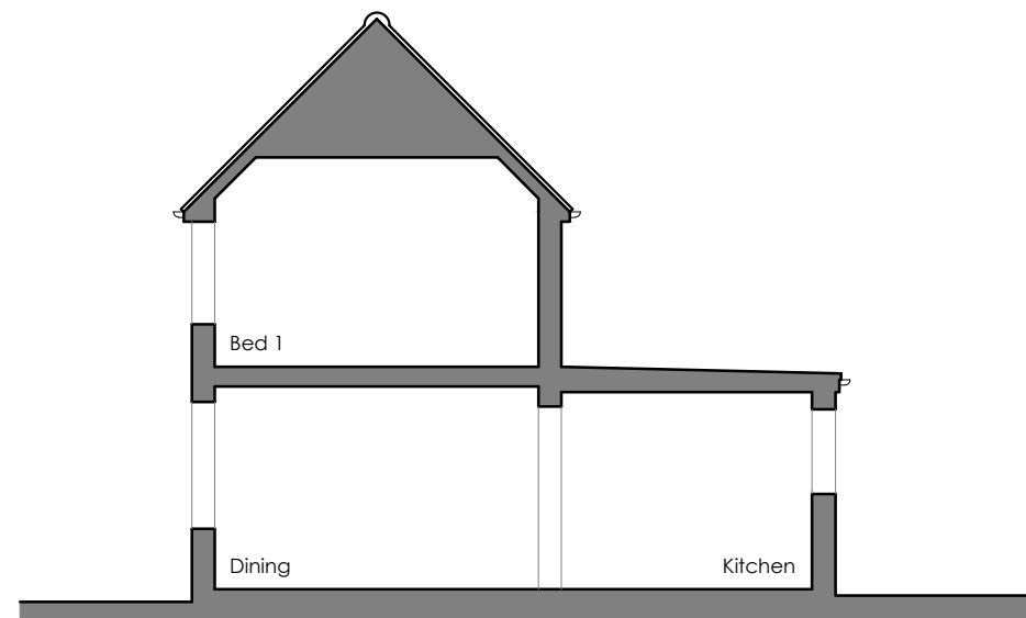
TYPICAL SECTION
