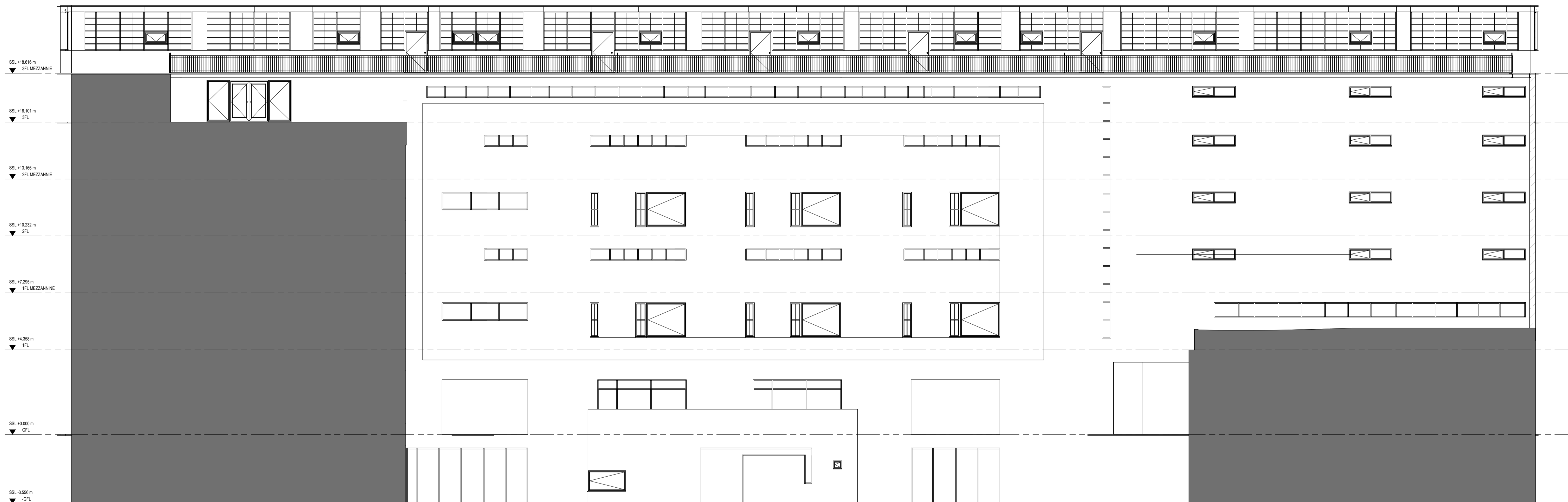
1 EXISTING EAST FACING INTERNAL COURT-YARD ELEVATION 1:100
