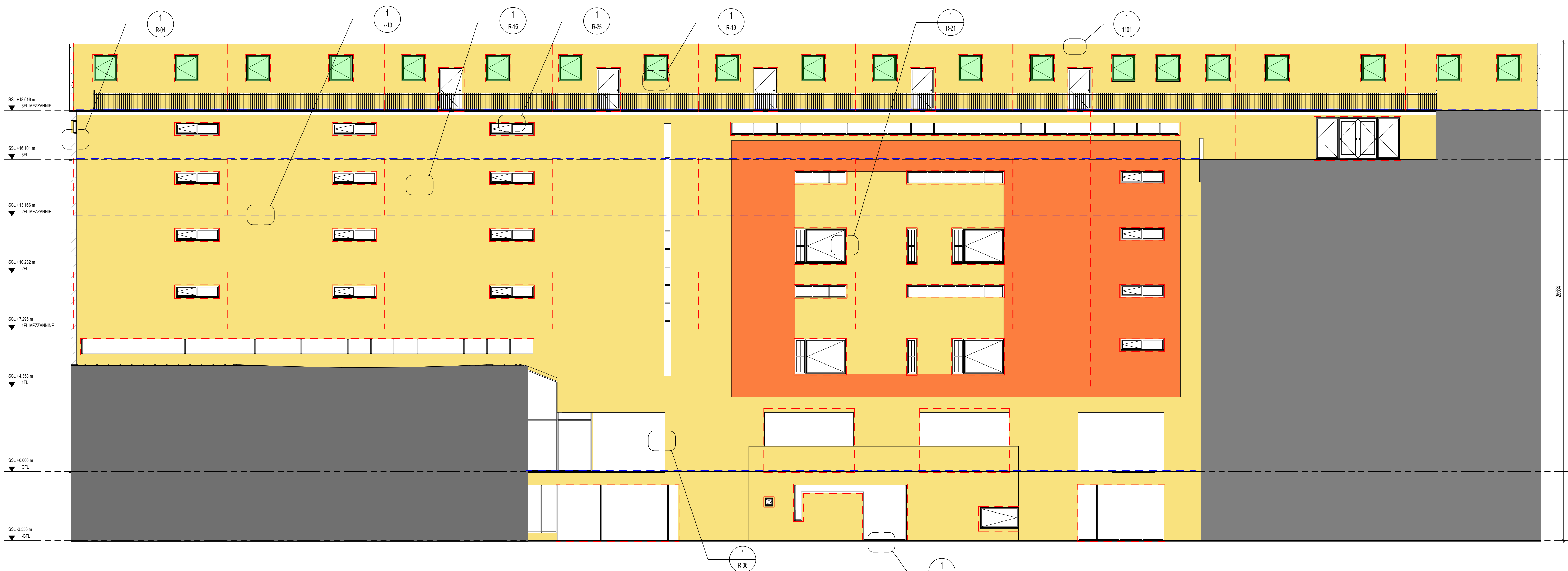
1 PROPOSED WEST FACING INTERNAL COURT-YARD ELEVATION 1:100
