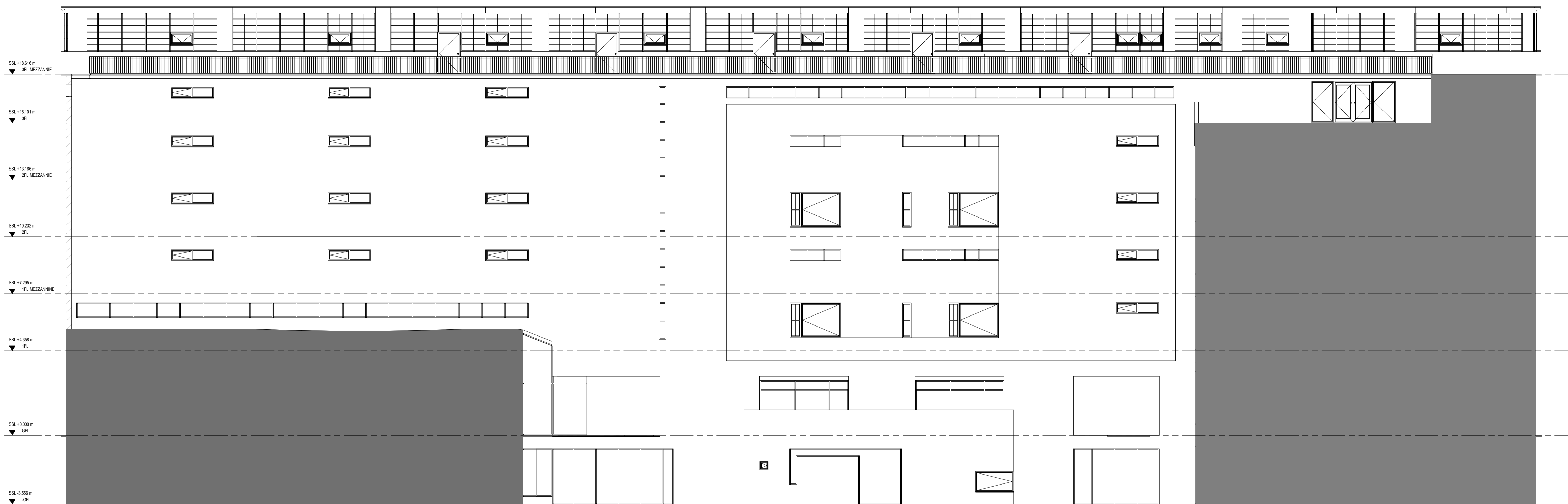
1 EXISTING WEST FACING INTERNAL COURT-YARD ELEVATION 1:100
