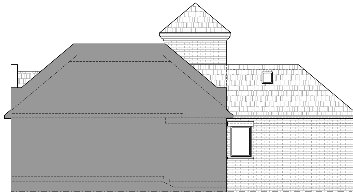
EXPROPOSED RIGHT SIDE ELEVATION
