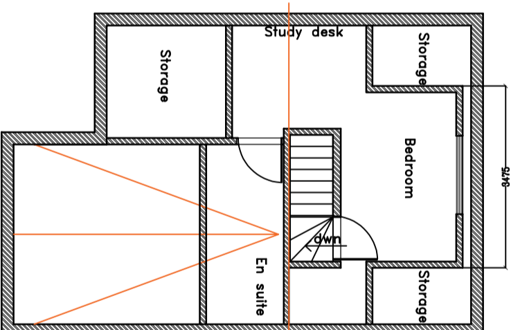
PROPOSED LOFT FLOOR PLAN
