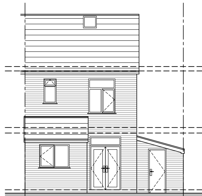
REAR ELEVATION 1:100
