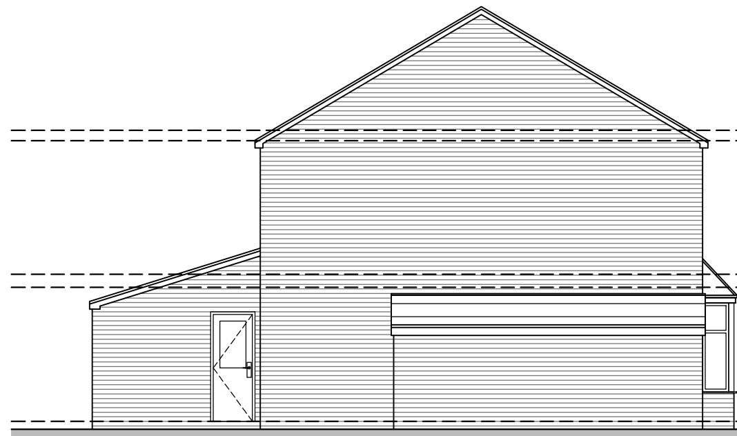
LEFT ELEVATION 1:100
