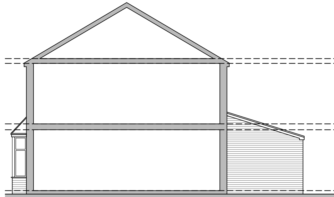
RIGHT ELEVATION 1:100
