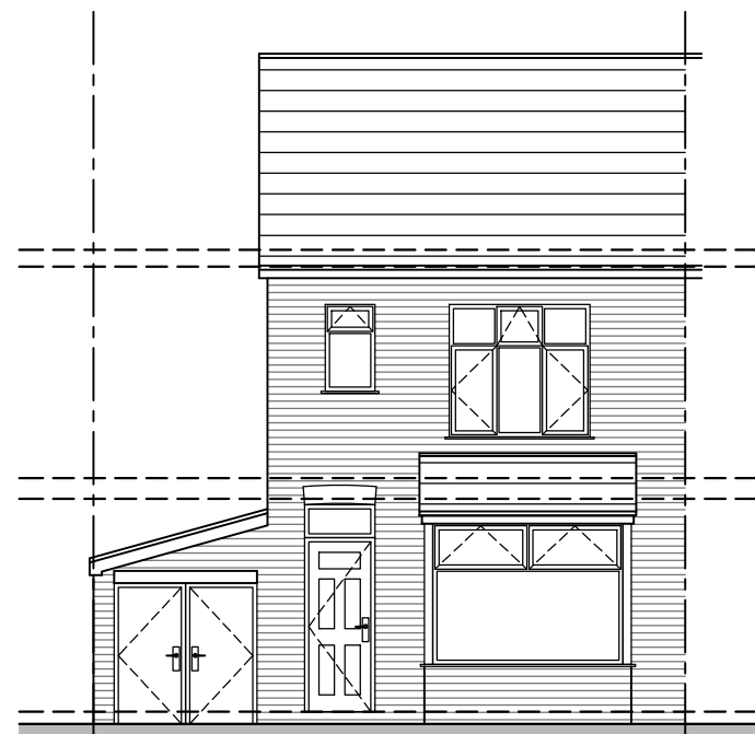
FRONT ELEVATION 1:100
