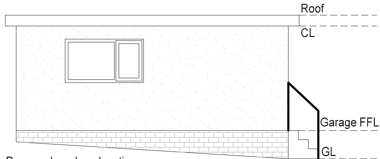
Proposed garden elevation
