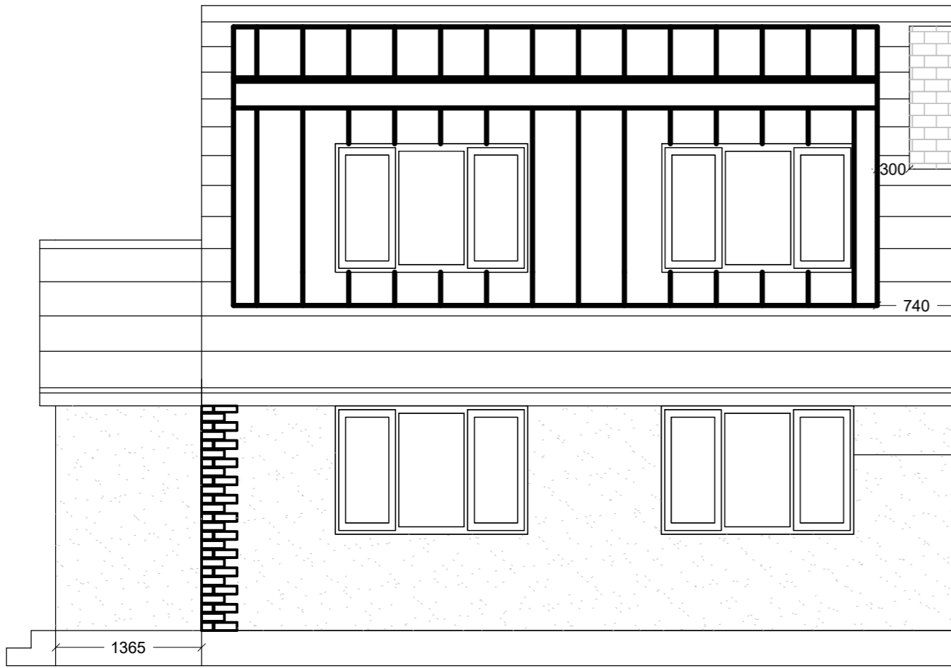
Proposed front elevation A3 1:50
