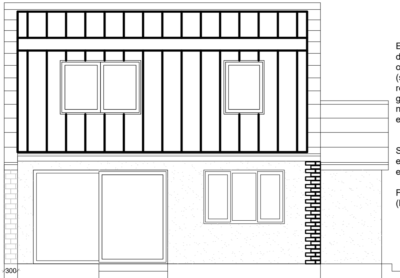
Proposed rear elevation A3 1:50
