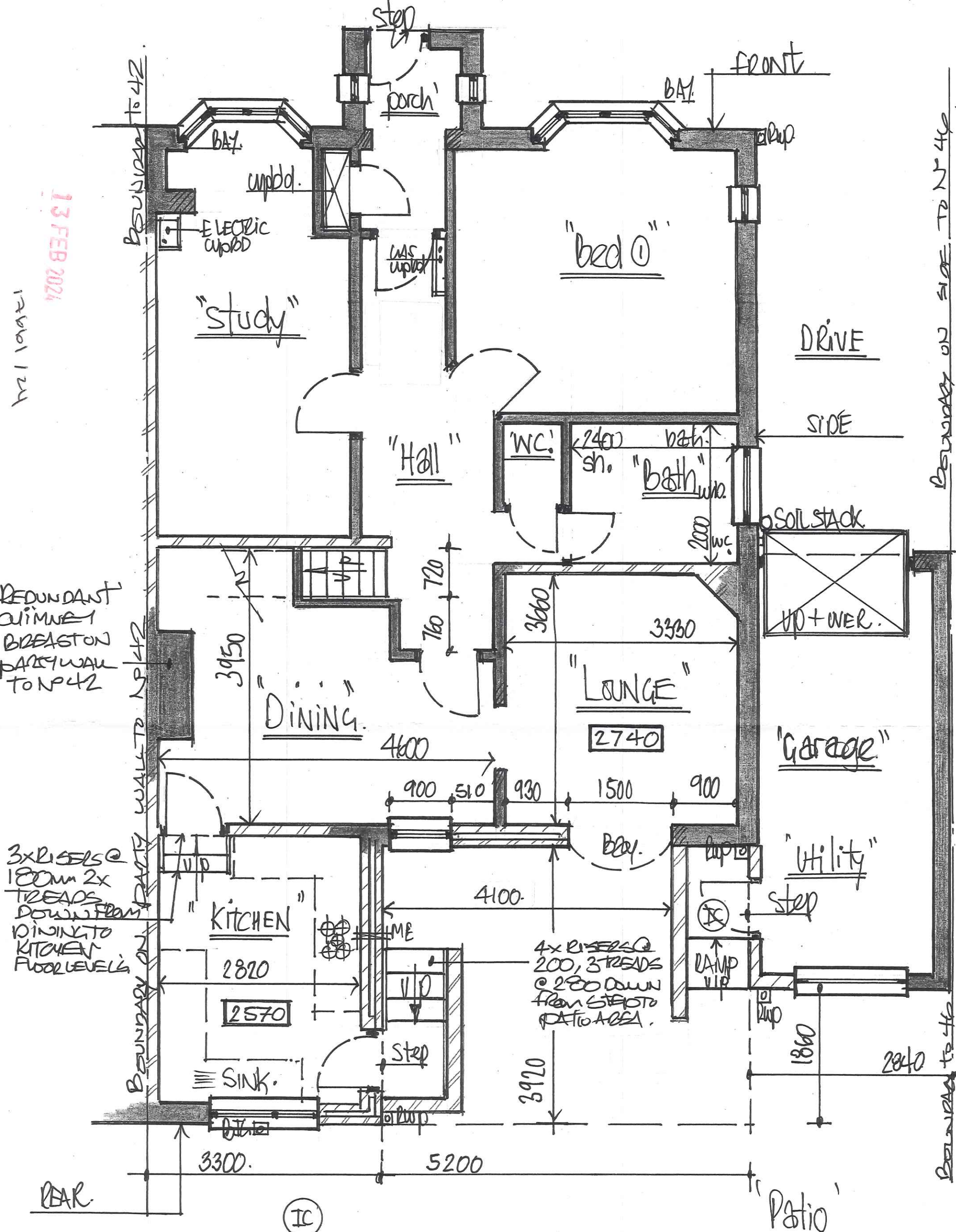
1:50 EXISTING "GROUND FLOOR" PLAN
