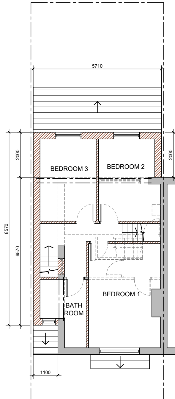
FIRST FLOOR 1:100
