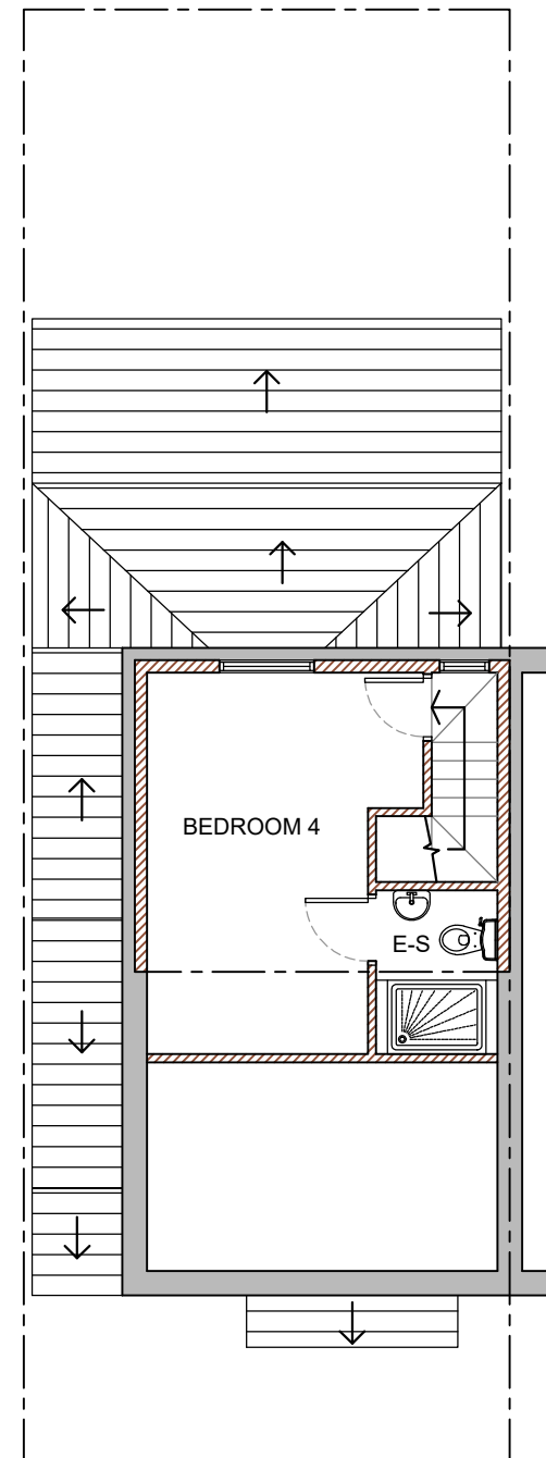
SECOND FLOOR 1:100
