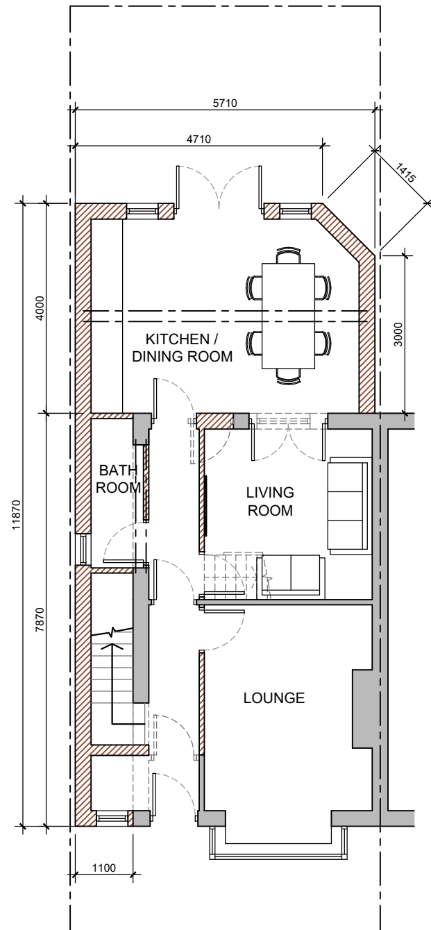
GROUND FLOOR 1:100
