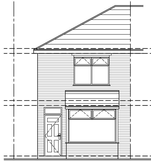
FRONT ELEVATION 1:100
