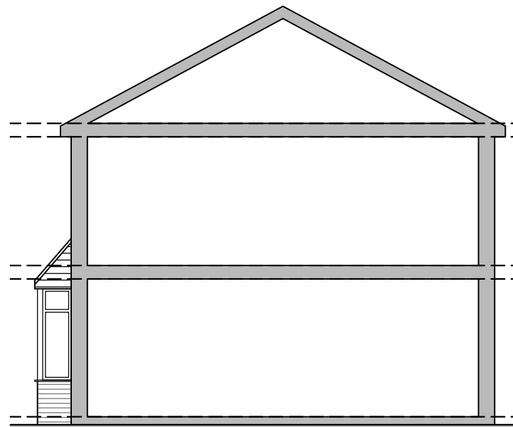
SIDE ELEVATION 1:100
