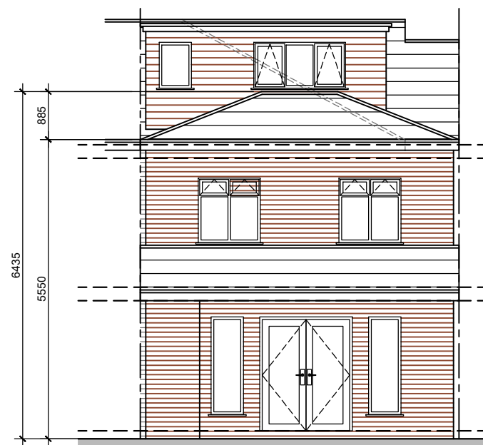
REAR ELEVATION 1:100
