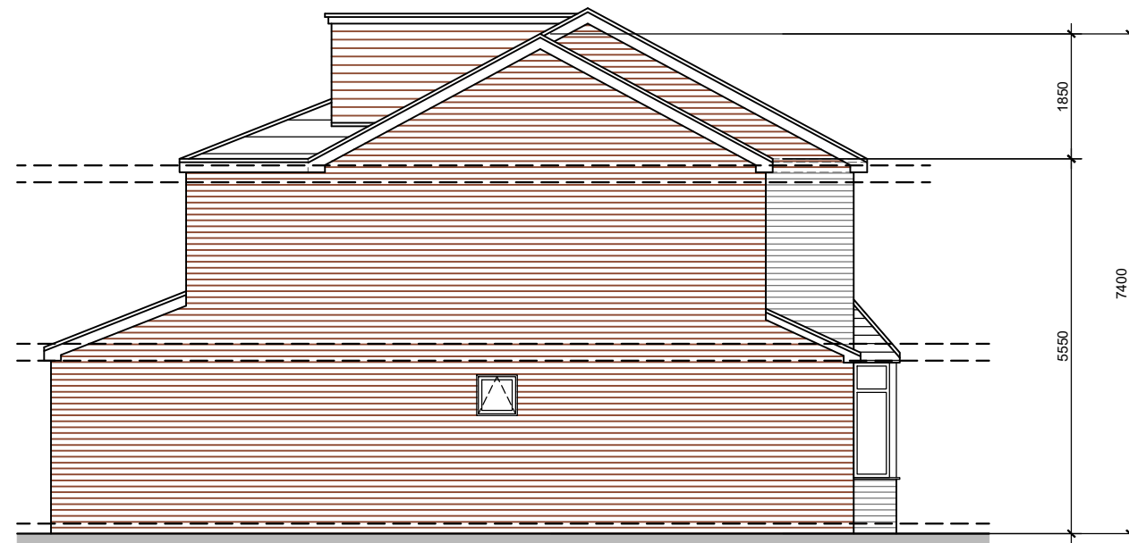
SIDE ELEVATION 1:100
