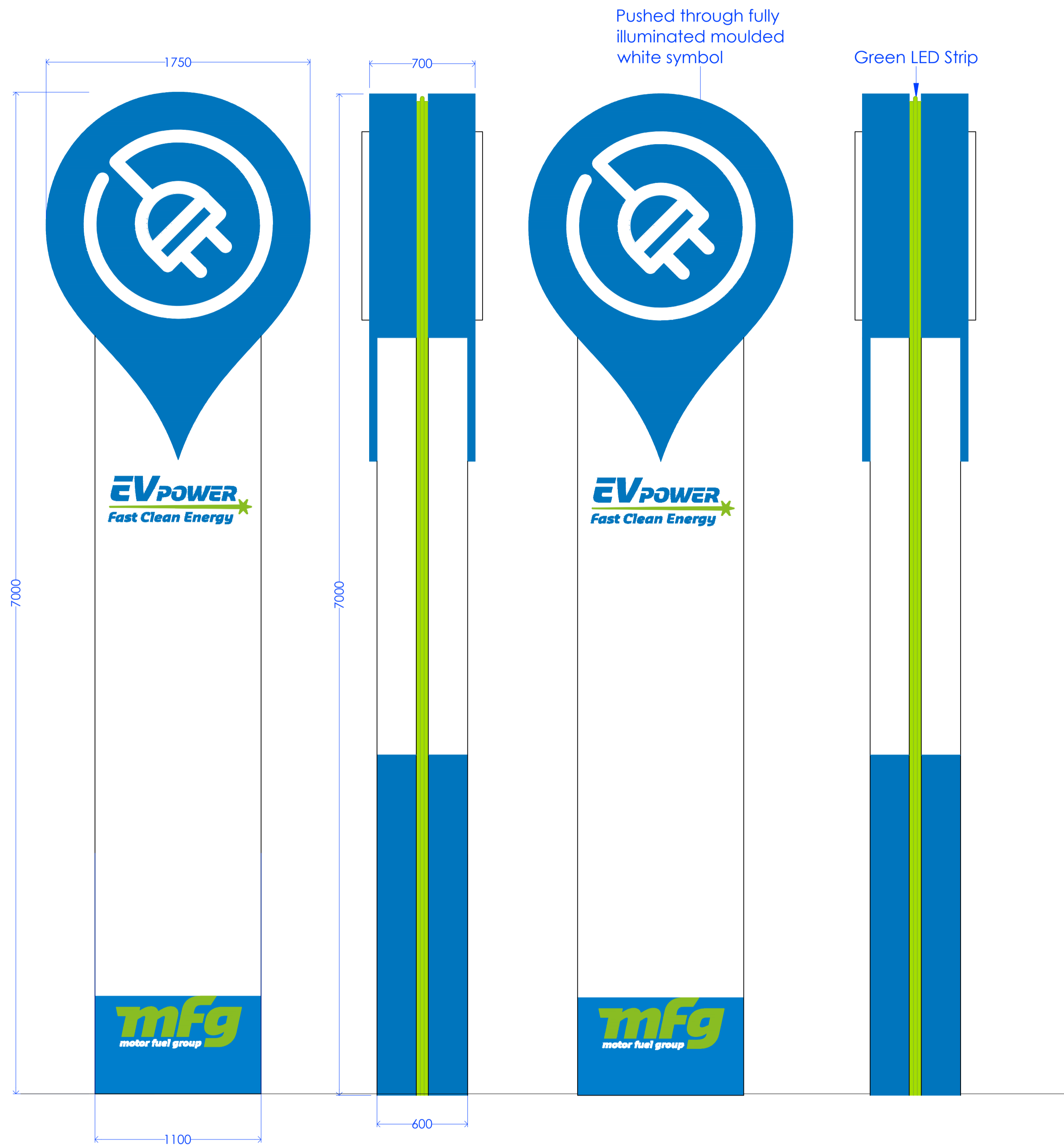
A - EV TOTEM DETAILS Scale 1:20
