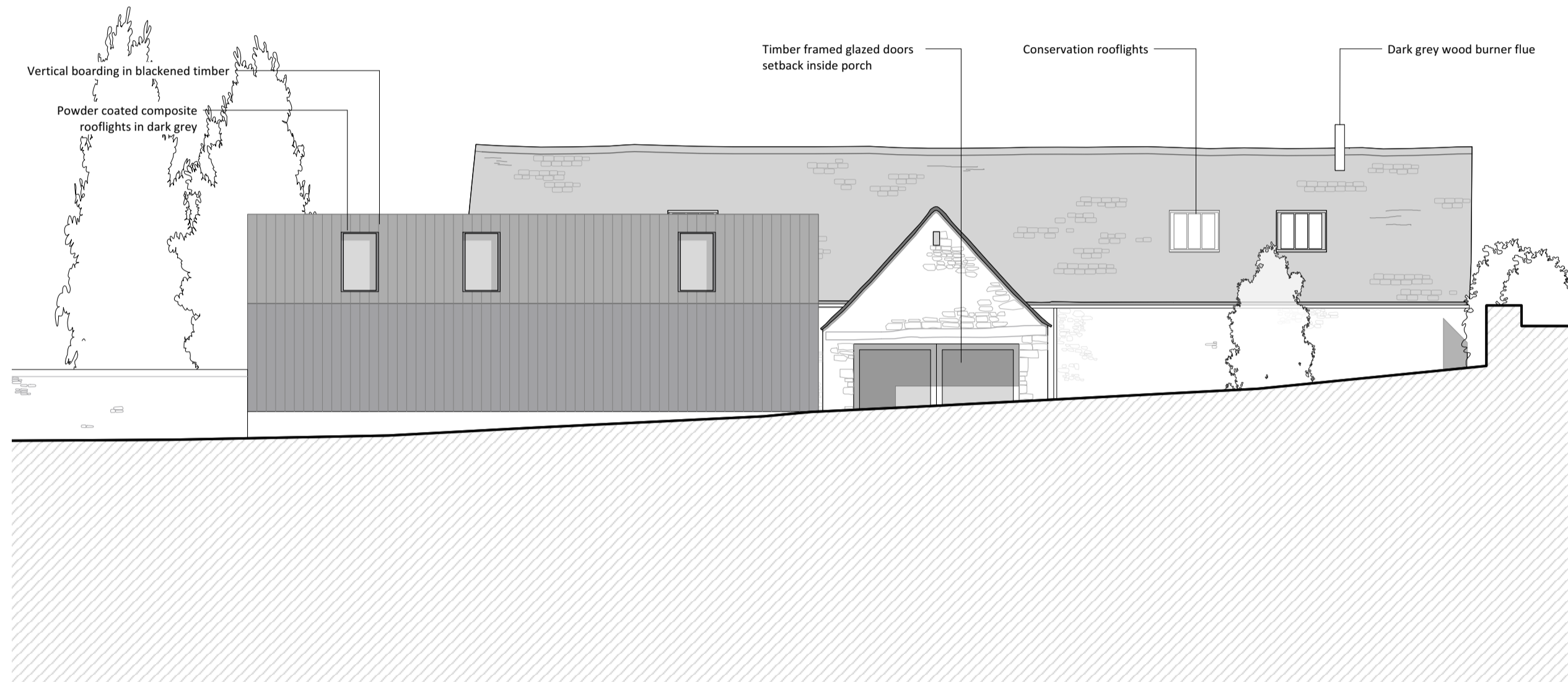
North-West Elevation
