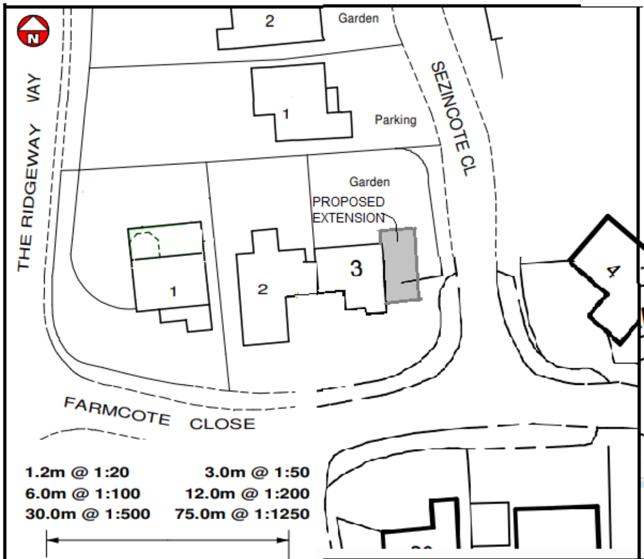
TORTONESE 3 FARMCOTE CLOSE EASTCOMBE PROPOSED BLOCK PLAN
