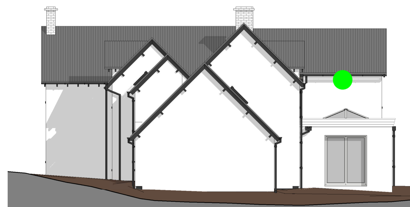
5 Proposed North Elevation 1 : 100
