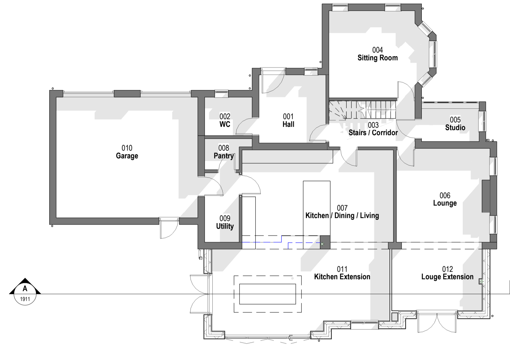
1 Proposed Ground Floor 1 : 100
