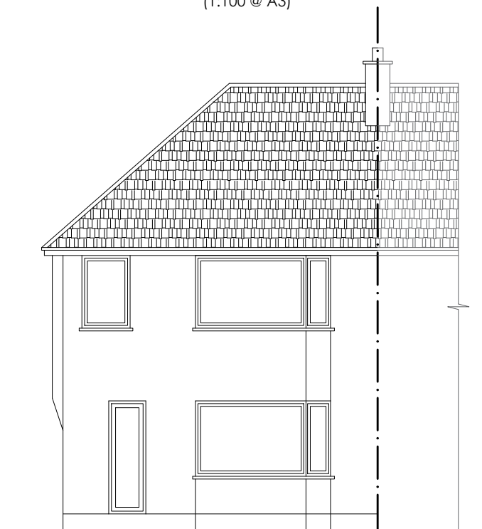
FRONT ELEVATION (1:100 @ A3)
