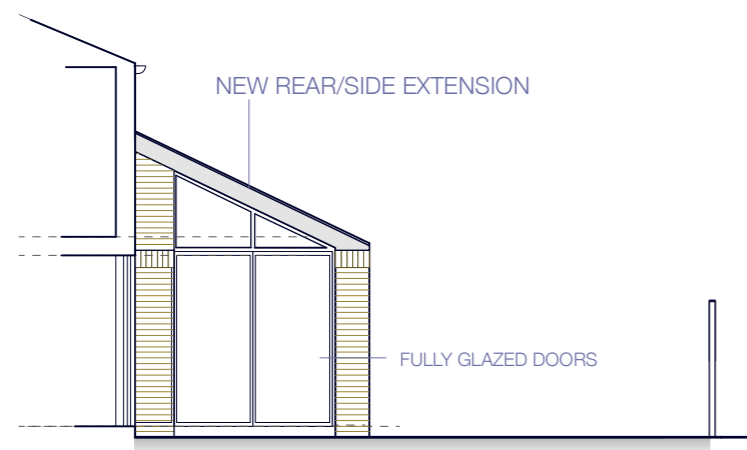
INNER COURTYARD ELEVATION
