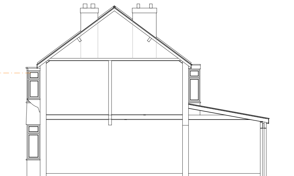
EXISTING SECTION 1:100
