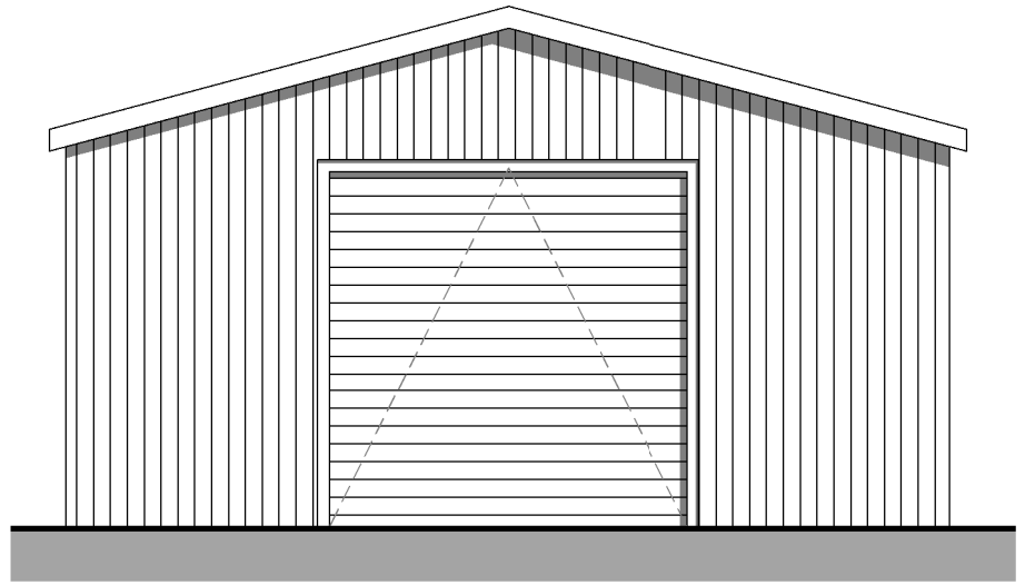
3 Pre-Existing Rear Elevation - Outbuilding 2314-A-202 1 : 50
