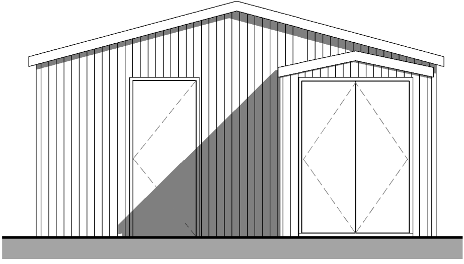
2 Pre-Existing Front Elevation - Outbuilding 2314-A-202 1 : 50
