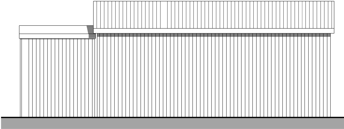
4 Pre-Existing Side Elevation - Outbuilding 2314-A-202 1 : 50
